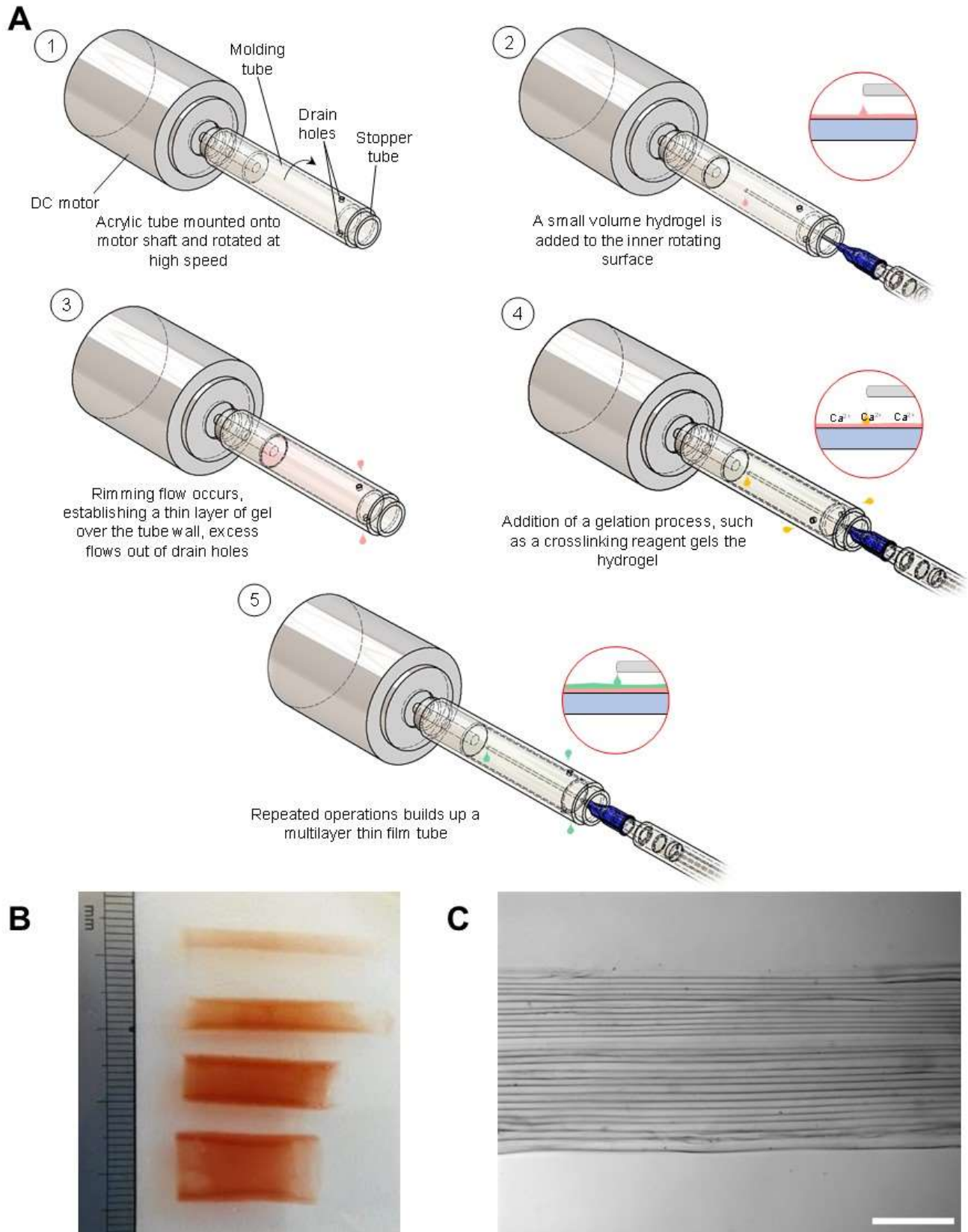
Figure 1. Illustration of RIFLE equipment and process. (A) Schematic representation of the RIFLE process. (B) Layered alginate tube size examples formed from moulds of different internal diameters, note: red food dye added to alginate to improve visualisation. (C) Brightfield microscopy image of a tube wall showing discrete alginate layers, white scale bar is 500 \mu m.
