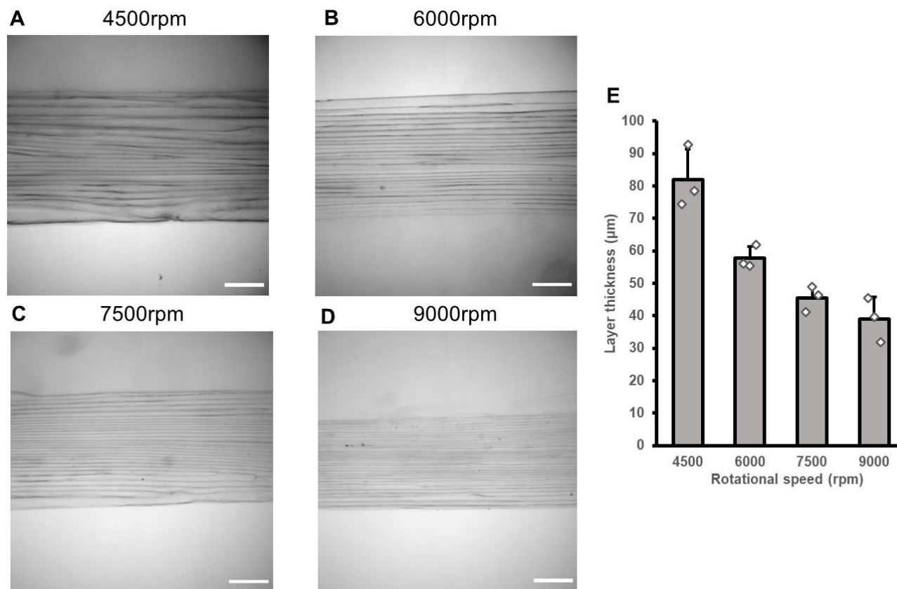
Figure. 2 - Layer thicknesses for RIFLE are determined by the speed of rotation. Brightfield microscopy images of tube walls formed using alginate 1% (W/V) at various rotational speeds. Scale bars are 500µm. (A) 4500rpm, (B) 6000rpm, (C) 7500rpm and (D) 9000rpm. (E) Plot of layer thicknesses for rotational speed variation. Mean with error bars \pm SD n=3.
