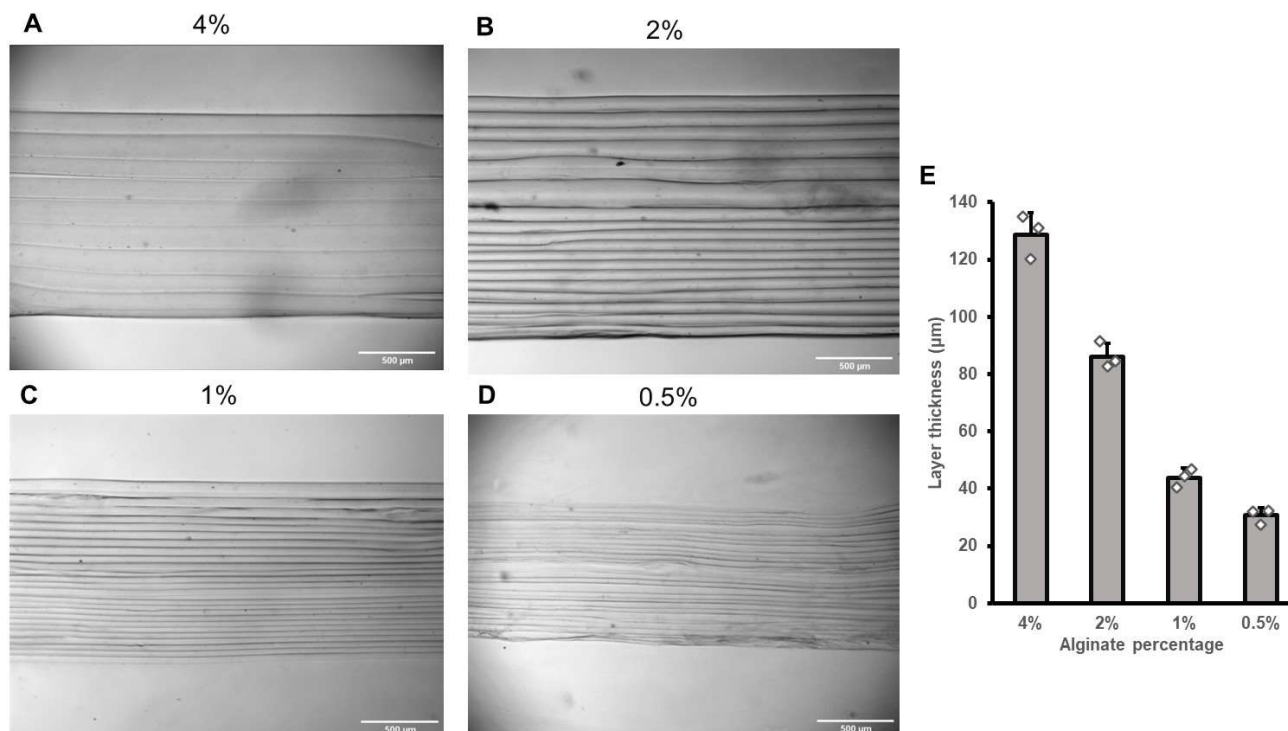
Figure. 3 – Algininate concentration influences the microscale layer thicknesses in tubes formed using RIFLE. Brightfield microscopy images of tubes walls with layer thicknesses and algininate concentration variation for tubes formed at 9000rpm. Algininate percentages (w/v) (A) 4%, (B) 2%, (C) 1% and 0.5%. Scale bars are 500µm. (E) Plot of layer thicknesses for algininate concentration variation. Mean with error bars \pm SD, n = 3.
