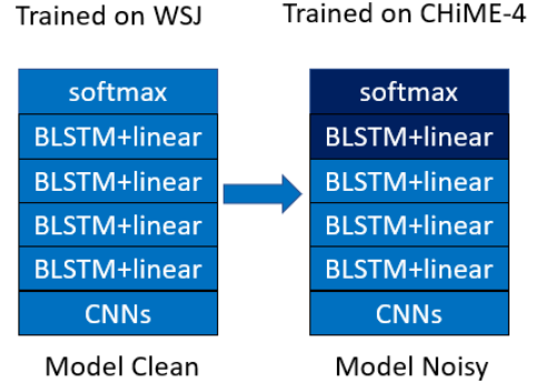
Fig. 1. An illustration of the transfer learning from WSJ to CHiME-4. Model Clean is trained on WSJ. Then, the top two layers (we group each BLSTM layer and its following linear layer as one layer) are either frozen or tuned with a small learning rates on the CHiME-4 noisy data. The bottom layers of Model Noisy are either random initialized or initialized using the weights of Model Clean, and trained on CHiME-4 with no learning rate re-scaling.
