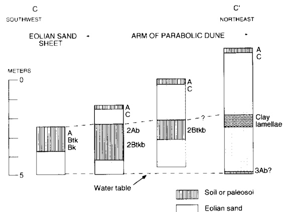
Fig. 5. Cross-section C–C' through eolian sands in an area south of the South Platte River in the Fort Morgan dune field. Location of section shown in Fig. 3.
