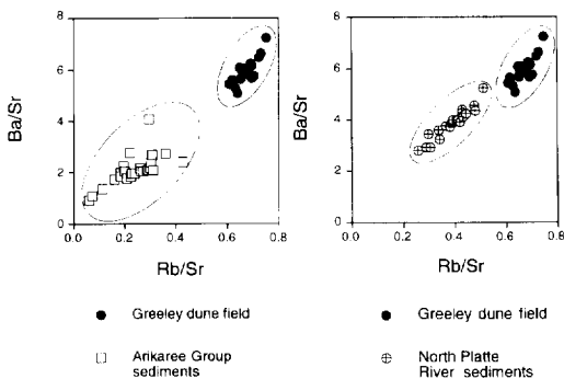
Fig. 18. Plots of Ba/Sr and Rb/Sr values for sands from the Greeley dune field, the Arikaree Group, and the North Platte River.
