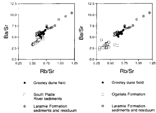
Fig. 19. Plots of Ba/Sr and Rb/Sr values for sands from the Greeley dune field, the Laramie and Ogallala Formations, and the South Platte River.
