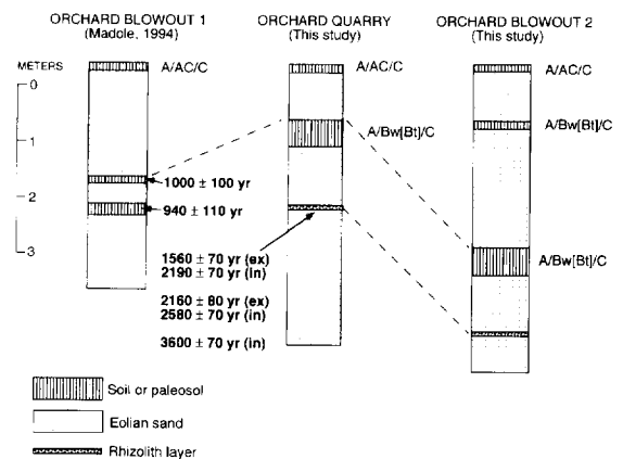
Fig. 10. Eolian stratigraphy exposed in a blowout and quarry exposures north of Orchard, Colorado in the Greeley dune field, showing radiocarbon ages of rhizoliths (this study) and soil organic matter (Madole, 1994).
