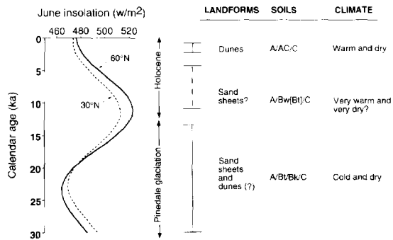
Fig. 22. Estimated times of eolian sand deposition in northeastern Colorado, inferred climates at the times of sand deposition and comparison to June insolation at the top of the atmosphere for latitudes bracketing the study area. Insolation data from Berger and Loutre (1991).
