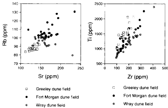
Fig. 14. Plots of Rb, Sr, Ti, and Zr contents for sands of the three dune fields in northeastern Colorado.
