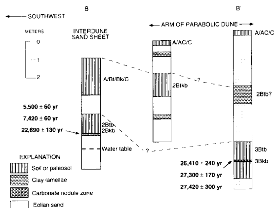
Fig. 4. Cross-section B–B' through eolian sands in an area south of the South Platte River in the Fort Morgan dune field; ages are from accelerator radiocarbon analyses of carbonate nodules. Location of section shown in Fig. 3.
