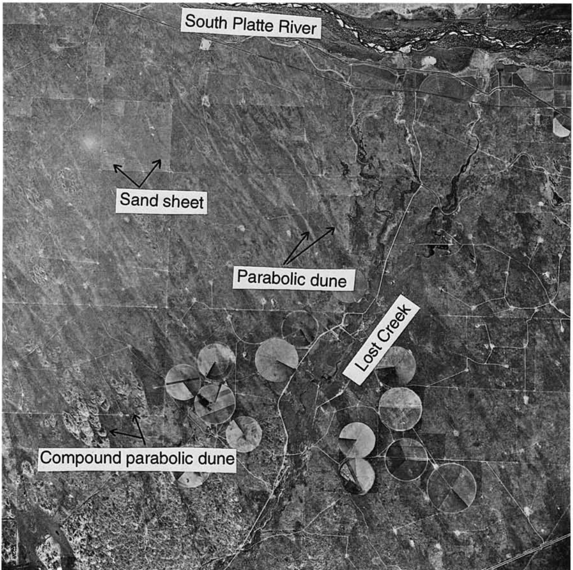
Fig. 2. Aerial photograph of the Lost Creek area south of the South Platte River (near the area mapped in Fig. 3) in the Fort Morgan dune field showing simple parabolic dunes, compound parabolic dunes, and sand sheets.
