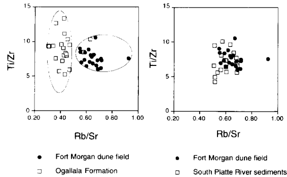
Fig. 16. Plots of Ti/Zr and Rb/Sr values for sands from the Fort Morgan dune field, the Ogallala Formation, and the South Platte River.
