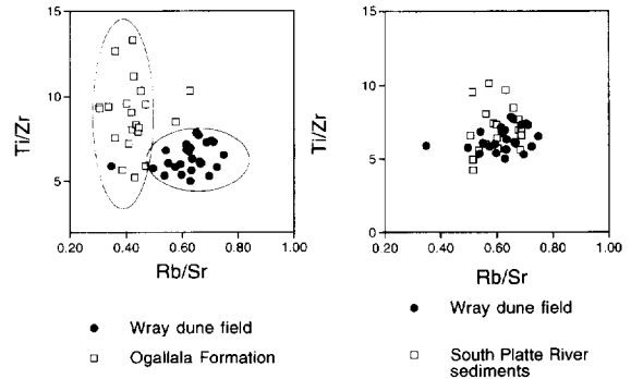
Fig. 17. Plots of Ti/Zr and Rb/Sr values for sands from the Wray dune field, the Ogallala Formation, and the South Platte River.
