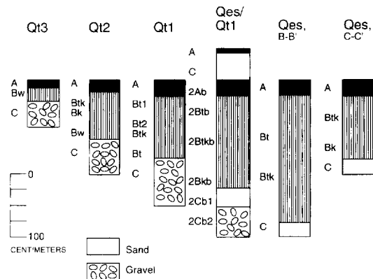
Fig. 8. Soil profile development in terrace alluvium along the South Platte River and in Osgood soils developed in interdune sheet sands south of the South Platte River at localities where cross-sections B–B' and C–C' were measured.
