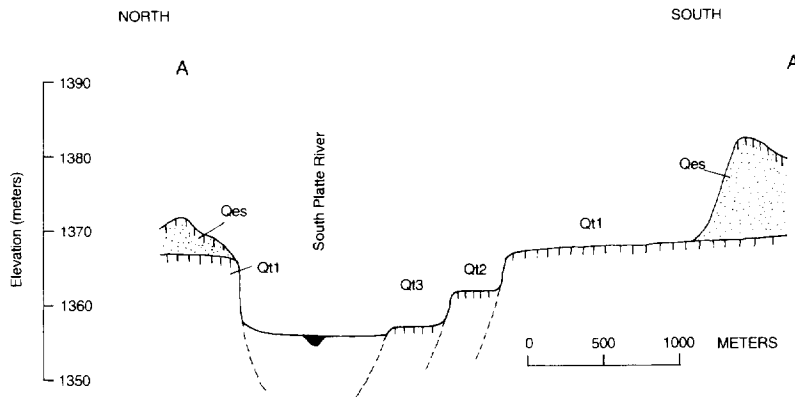
Fig. 6. Cross-section A–A' north and south of the South Platte River between Greeley and Fort Morgan, Colorado. Location of section shown in Fig. 3.
