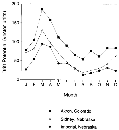
Fig. 20. Plot of monthly values of drift potential (DP) for three localities adjacent to northeastern Colorado dune fields.
