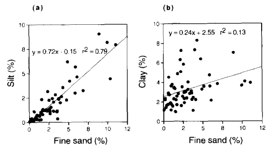
Fig. 13. Plots of silt content as a function of fine-sand content, and clay content as a function of fine-sand content in eolian sands in northeastern Colorado.
