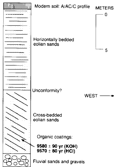
Fig. 9. Eolian sediments exposed in the Logan County landfill near Sterling, Colorado, in the Fort Morgan dune field, and radiocarbon ages of organic coatings on grains found in foreset beds.
