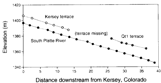
Fig. 7. Longitudinal profiles of the South Platte River and the Kersey and Qt1 terraces downstream from Kersey, Colorado. Downstream distances in kilometers.
