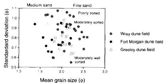
Fig. 11. Mean grain size and sorting values for eolian sands from three dune fields in northeastern Colorado.
