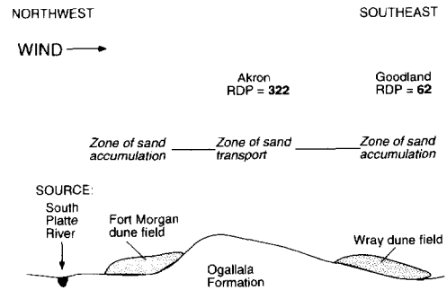
Fig. 23. Schematic cross-section D-D' (location shown in Fig. 1) from the South Platte River near Sterling, Colorado, to the Wray dune field near Wray, Colorado, showing locations of dune fields relative to the Ogallala caprock upland, and RDP values for selected localities.
