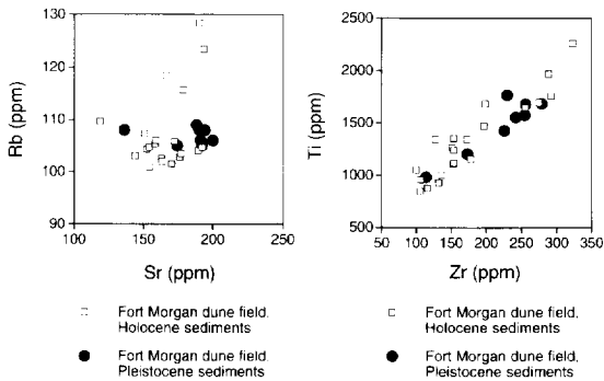
Fig. 15. Plots of Rb, Sr, Ti, and Zr contents for Holocene vs. Pleistocene eolian sands from the Fort Morgan dune field.
