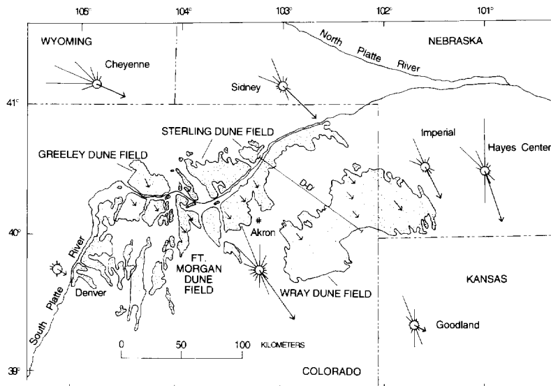
Fig. 1. Map showing distribution of eolian sand in northeastern Colorado and southwestern Nebraska, location of cross-section D–D' (Fig. 23), orientation of late Holocene paleowinds, and modern sand roses (calculated using the method of Fryberger and Dean, 1979). Eolian sand distribution west of 104° and north of 40° and all areas east of 102° were mapped by the authors; other areas are from Scott (1978), Sharps (1980), and Bryant et al. (1981).
