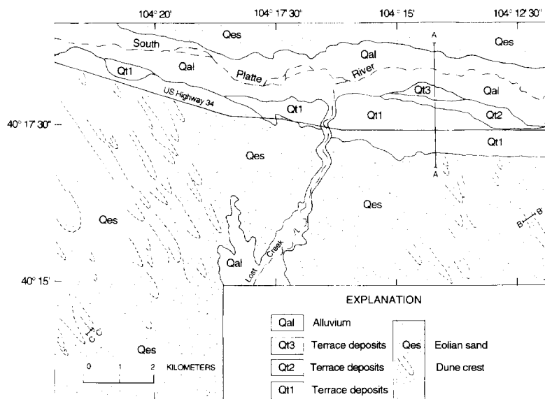
Fig. 3. Surficial geologic map of a portion of the Lost Creek area south of the South Platte River, between Greeley and Fort Morgan, Colorado, with locations of cross-sections shown in Figs. 4, 5 and 8.
