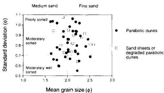
Fig. 12. Comparison of mean grain size and sorting values for parabolic dunes and eolian sand sheets in northeastern Colorado.
