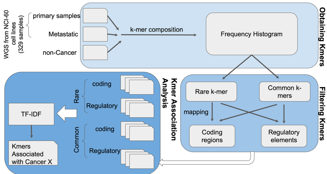
Figure 6. K-var workflow. The k -mer composition of whole-genome sequencing (WGS) sequencing data from cases and controls is obtained using Jellyfish. Rare and common k -mers are identified based on their frequency across samples, and mapped to a reference genome to assess their putative functional impact. Selected k -mers are then compared between cases and controls using term frequency-inverse document frequency (TF-IDF) statistical modeling to evaluate association with the phenotype of interest. As a proof of concept, K-var was implemented using cancer samples from the NCI-60 dataset.
