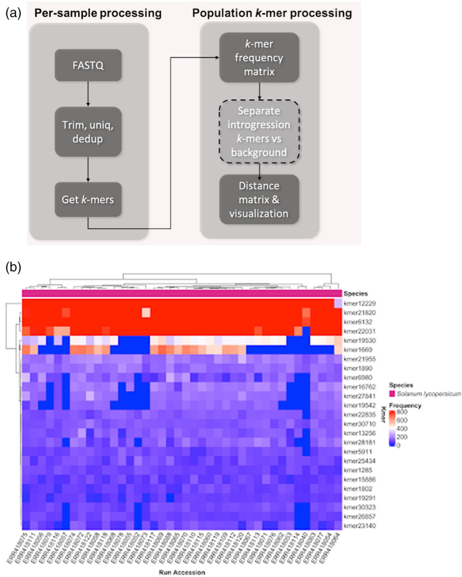
Figure 2. (a) kTom workflow, with major steps for individual sample and population data processing. (uniq = get unique reads; dedup = deduplicate reads). (b) k-mer frequency heatmap from kTom. Frequency of selected k-mers in each accession analyzed. Differential k-mer frequencies are apparent in this view. Depending on the nature of the accessions, this view may provide a first glimpse into genetic sequences underlying structural variations that differentiate the accessions.
