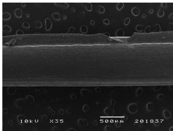
Figure 4 Representative SEM micrograph (35×) showing the middle portion of an Obturator. The superficial aspect is smooth with a longitudinal groove running from the tip to the coronal portion of the gutta-percha.
