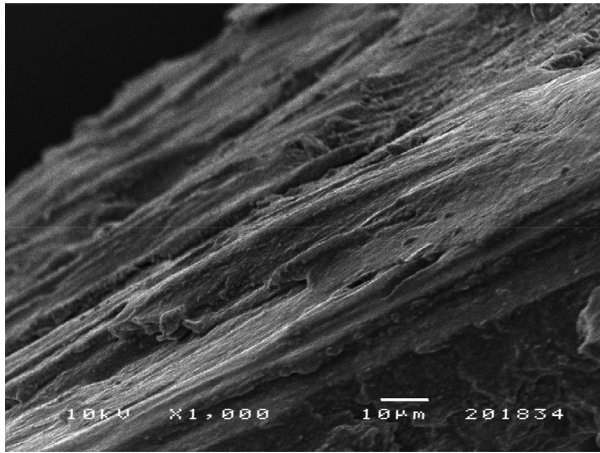
Figure 5 SEM micrograph (1000×) showing the outer surface of an Obturator. The superficial aspect is characterised by gutta-percha grooves oriented in parallel.
