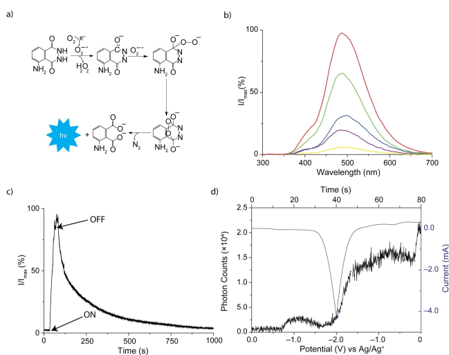
Figure 1. (a) Proposed mechanism for luminol cathodic ECL. [4a,16] (b) ECL of luminol ( 1.0 \times 10^{-3} M) in [EMIM][EtSO 4 ], recorded at a platinum mesh electrode biased at either -1.0 V (violet line), -1.5 V (yellow line), -2.0 V (blue line), -2.5 V (green line) and -3.0 V (red line). Spectra are normalized to the maximum intensity of the -3.0 V data set. (c) Time-resolved emission spectra (490 nm). The ON label indicates when the working electrode voltage bias is switched from open-circuit to -2.5 V. The OFF label indicates the end of the 30 s voltage pulse. (d) Photon counting experiments of luminol ECL during a cyclic voltammogram (the voltage was swept from 0.0 V towards -2.0 V, and back, at a scan rate of 0.05 V/s). Overlay plot of simultaneously acquired photon counts and current trace.
