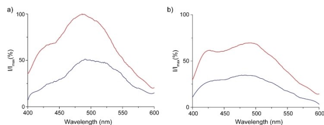
Figure 2. Electrogenenerated chemiluminescence of luminol ( 1.0 \times 10^{-3} M) in [EMIM][EtSO 4 ], obtained using a platinum mesh biased at either -2.5 V (blue line) or at -3.0 V (red line). The RTIL is deliberately spiked with water [5% v/v (a); 10% v/v (b)]. A further increase of water concentration to 15% v/v quenches completely the emission. Spectra are normalized to the maximum intensity of the -3.0 V, 5% v/v water data set.
