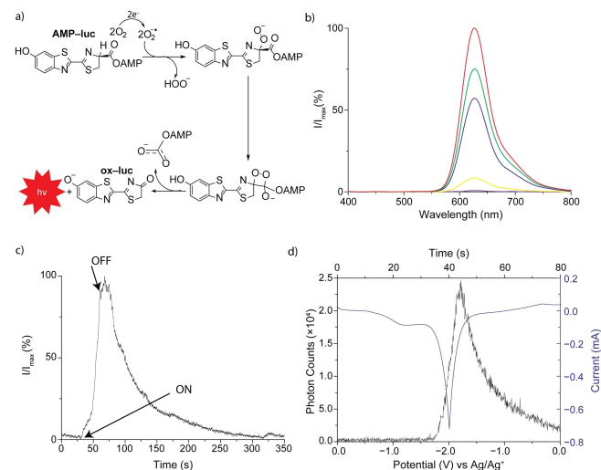
Figure 4. (a) Proposed mechanism for the firefly's luciferin ECL (extended mechanism in Figure S5). [9] (b) ECL of AMP-luc ( 4.3 \times 10^{-4} M) in [EMIM][EtSO 4 ] at a platinum mesh electrode biased at either -1.0 V (violet line), -1.5 V (yellow line), -2.0 V (blue line), -2.5 V (green line) and at -3.0 V (red line). Spectra are normalized to the maximum intensity of the -3.0 V data set. (c) Time-resolved emission spectra (626 nm). The ON label indicates the time at which the working electrode voltage bias is switched from open-circuit to -2.5 V. The OFF label indicates the end of the 30 s ( -2.5 V) voltage pulse. (d) Photon counting experiments of AMP-luc ECL during a cyclic voltammogram (the voltage was swept from 0.0 V to -2.0 V, and back, at a scan rate of 0.05 V/s).
