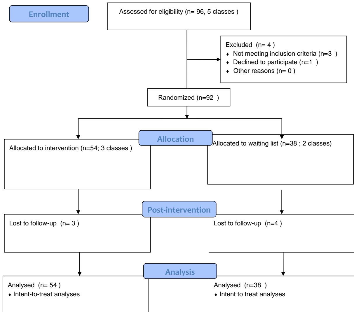
Figure 1. Study Flowchart
