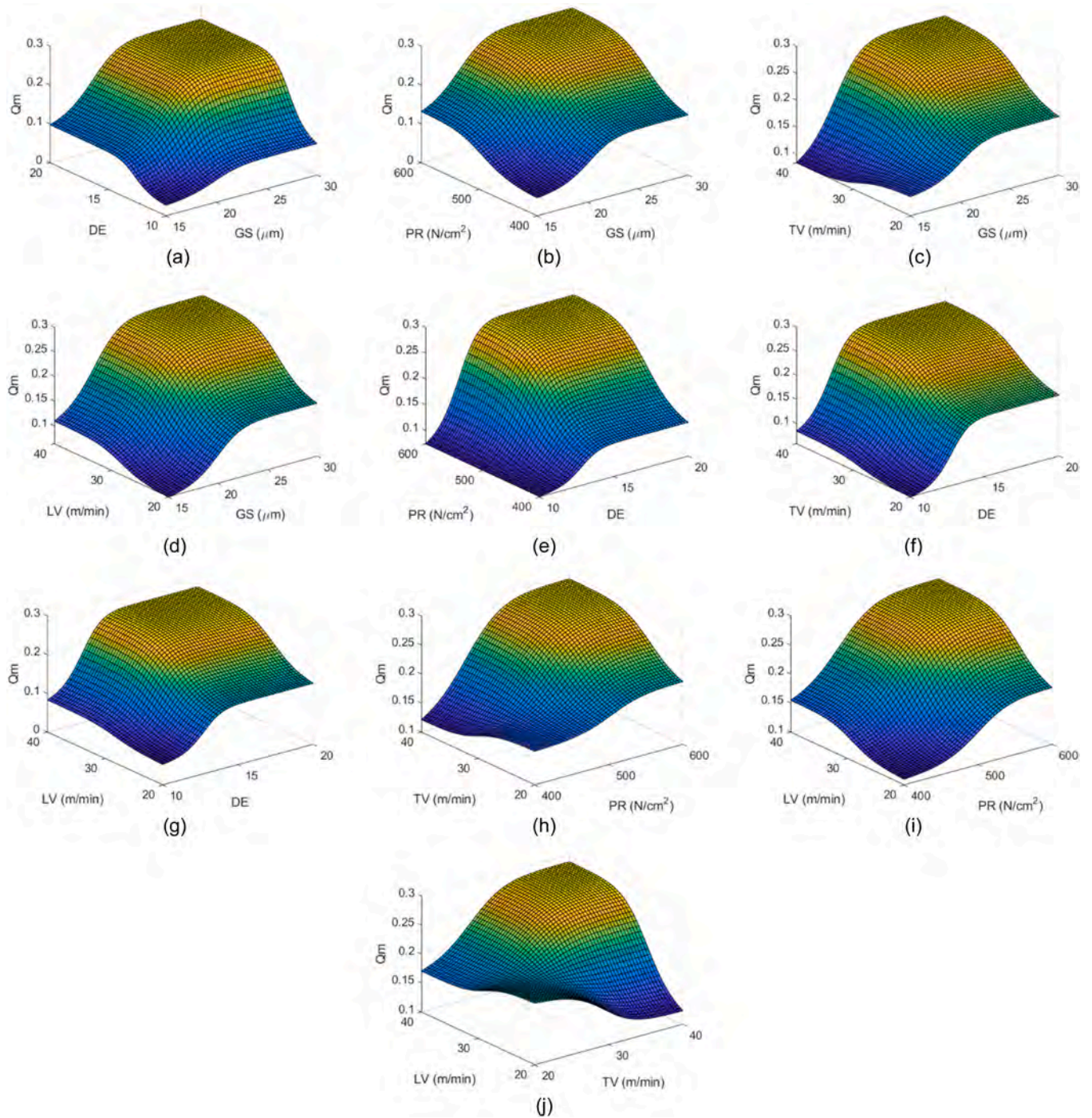
Fig. 14. Response surface for Q_m (cm/min) versus each pair of input variables while the rest are kept at their central values, using the ANFIS developed for Q_m : a) DE vs GS, b) PR vs GS, c) TV vs GS, d) LV vs GS, e) PR vs DE, f) TV vs DE, g) LV vs DE, h) TV vs PR, i) LV vs PR, j) LV vs TV.
