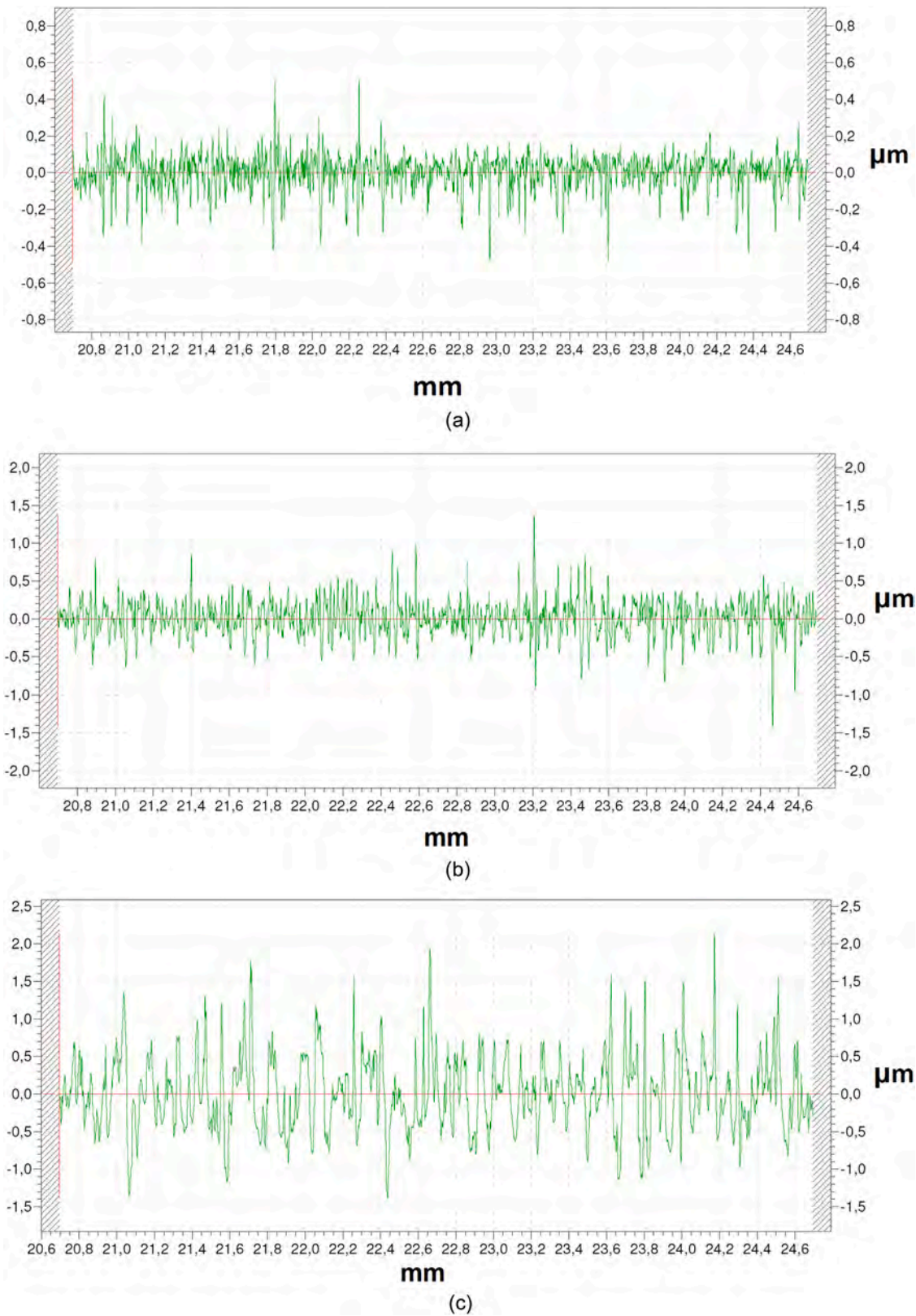
Fig. 7. Examples of roughness profiles for: a) grain size 15, b) grain size 20, c) grain size 30.
