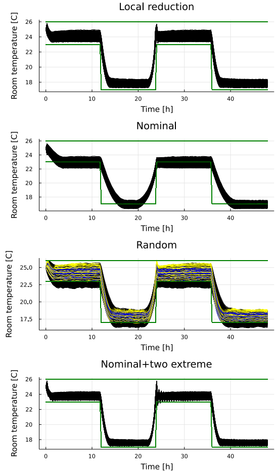
Figure 1: Comparison with other scenario-based approaches
