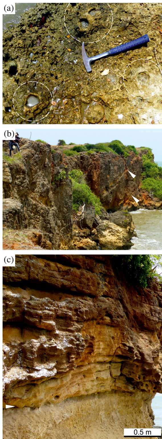
FIGURE 4 Shallow-marine facies. (a) Calcareous sandstone with abundant Ophiomorpha burrows (dashed circles), Bed 1. (b) Large NE-inclined clinoformal foresets (white arrow heads) exposed on the sea cliff at Point Kudrimalai, Bed 2. In contrast, Miocene limestone occurrences in NW coastal Sri Lanka are horizontally bedded. (c) Sharp contact (white arrow head) between the bioturbated calcareous sandstone of bed 1 and the internally laminated sandstone foresets of Bed 2. This outcrop shows a horizontal bedding since it cuts the inclined beds parallel to strike [Colour figure can be viewed at wileyonlinelibrary.com ]
