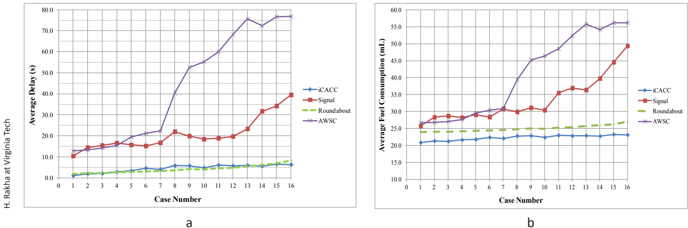
Figure 2. Comparison Between Different Scenarios (a) Average Delay Comparison per Vehicle (seconds) (b) Average Fuel Consumption per Vehicle (milliliters)
