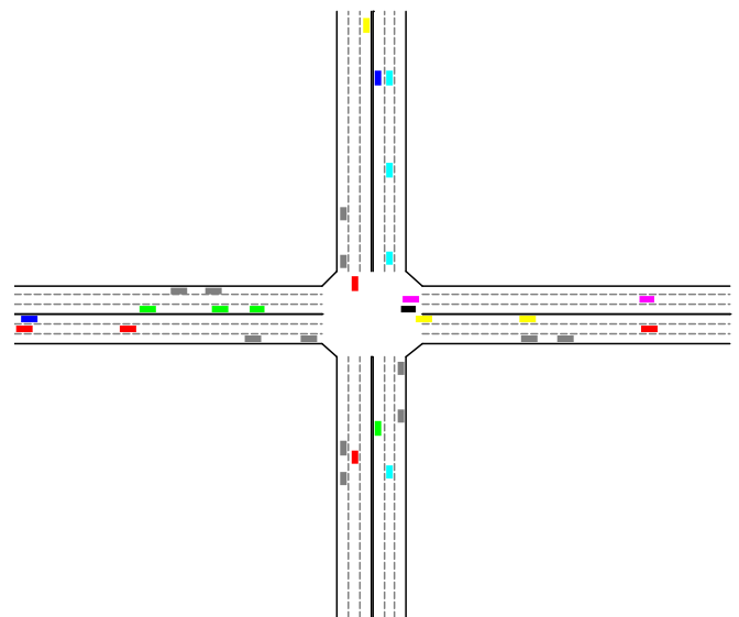
Figure 1. A Screen Shot From the iCACC Used for Simulating Advanced Vehicles.
