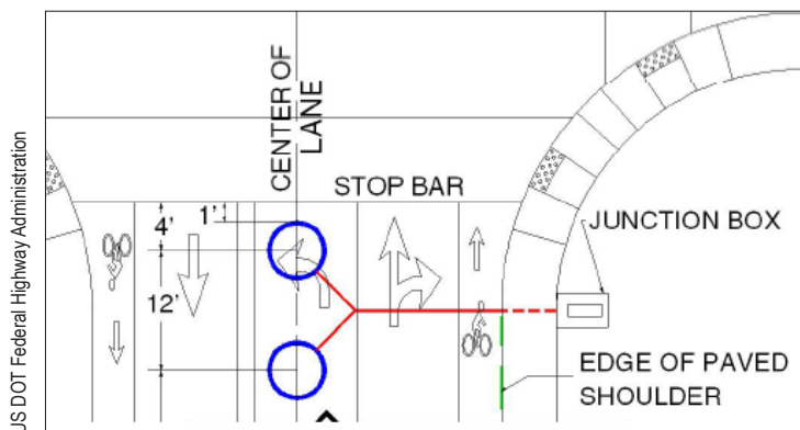
Figure 1. Traditional loop detector schematic
