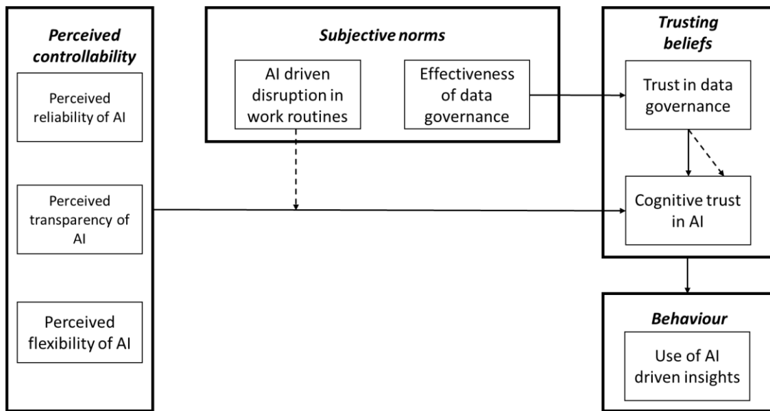
Figure 1. Proposed framework
