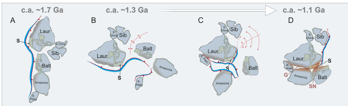
Fig. 1. Schematic plate reconstruction of the amalgamation of Rodinia from 1.7 Ga to 1.1 Ga based on the reconstructions of Li et al. (2008), Cawood and Pisarevsky (2017) and Martin et al. (2020). Laur = Laurentia, S = Scotland, S China = South China Craton, Sib = Siberian craton, Balt = Baltica, R. Plata = Rio de la Plata craton, G = Grenville orogeny, SN = Sveeno-norwegian Orogeny. Dark blue with red trim = subduction (red teeth indicate hanging-wall side), double ended red arrows = ocean spreading, red/orange shading = ~1.1 Ga orogenesis. (For interpretation of the references to colour in this figure legend, the reader is referred to the web version of this article.)
