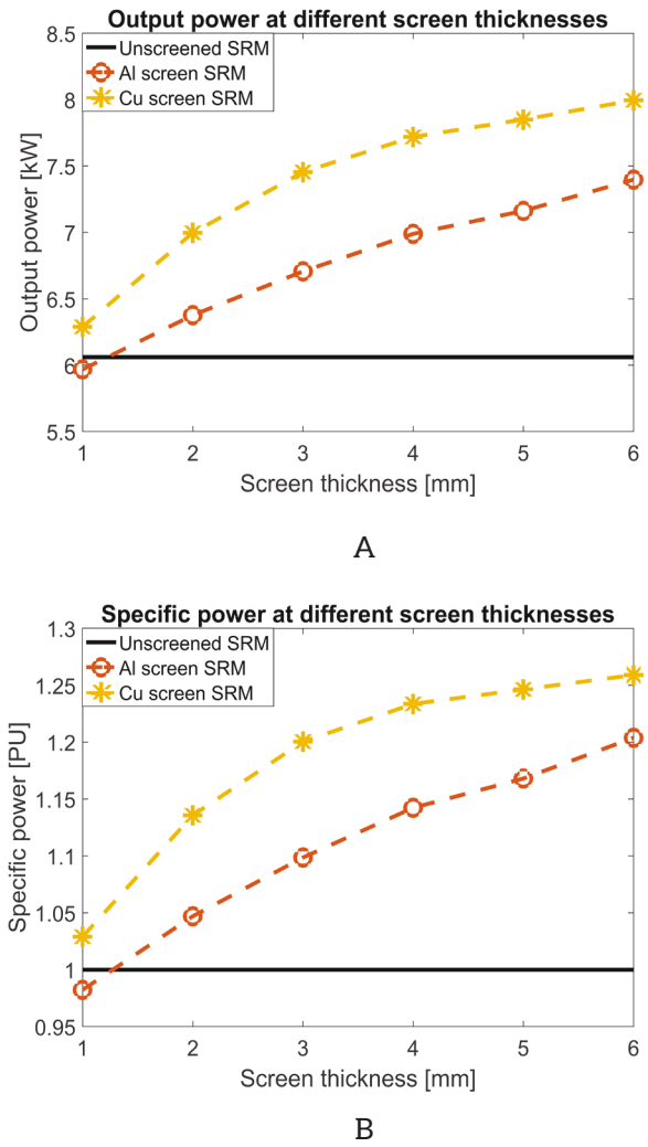
Fig. 14. Performance comparison of unscreened and screened SRMs: (a) output power and (b) specific power
