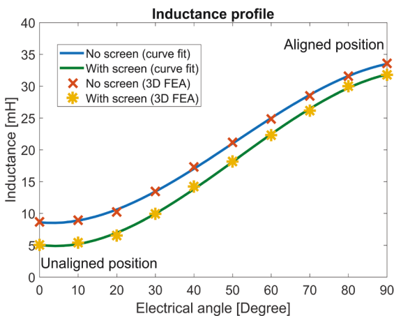
Fig. 8. Inductance profile
