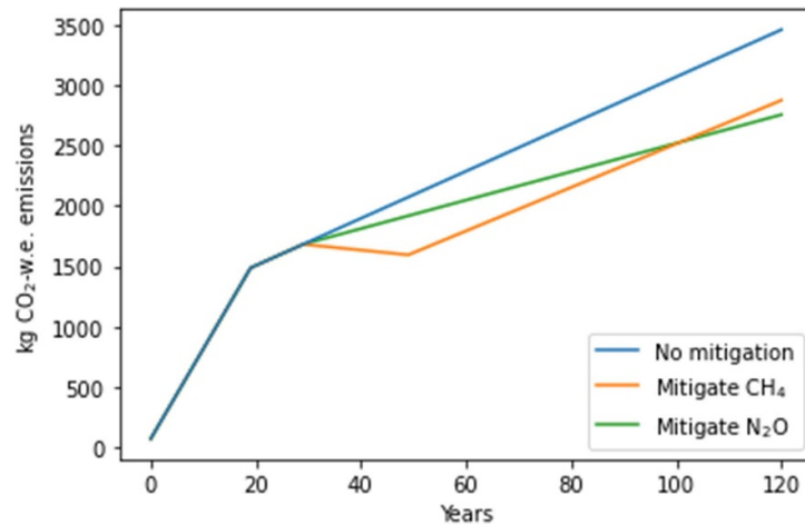
Figure 8. Hypothetical virtual experiment to determine which GHG (i.e. CH 4 or N 2 O) would be more appropriate to mitigate at year 30 over a 100 years time horizon. w.e. = warming equivalent.
