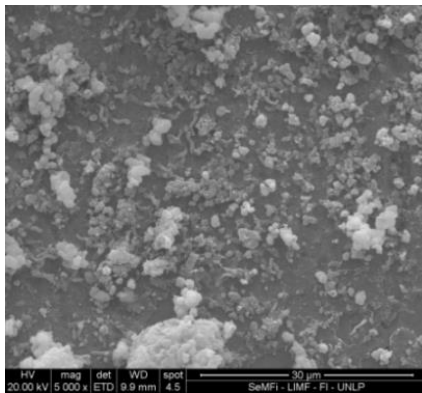
Fig. 1: SEM image of SRB biofilm formation on SAE 1010 carbon steel coupon after 7 days of incubation.
