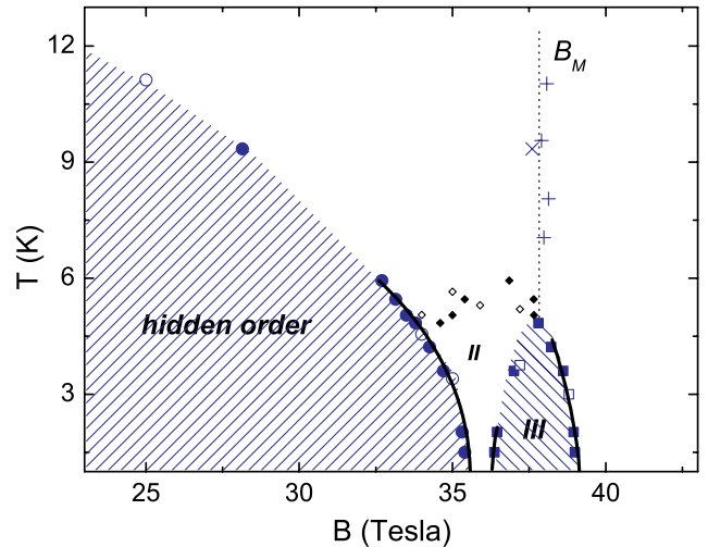
FIG. 4 (color online). Temperature-magnetic-field phase diagram. Open (closed) symbols were extracted from thermal-expansion (magnetostriction) experiments. \times (+) denotes the metamagnetic transition B_M from this work (from Ref. [16]). Bold solid lines correspond to clear first-order phase transitions.
