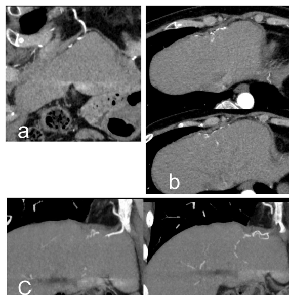
Fig. 3 The right internal thoracic artery was connected to the intrahepatic artery through Sappey’s superior artery on the coronal (a), axial (b), and oblique (c) post-ET CTA images in case 5
