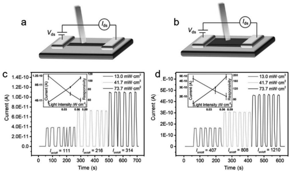
Fig. 2. Structure of photodetectors based on \text{MAPbI}_3 nanowires (A) and nanoplates (B) [25]
