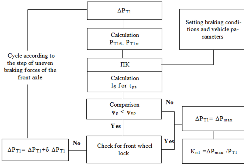
Fig. 5. Algorithms for determining the permissible uneven braking forces on the wheels of the front axle
