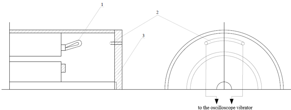
Fig. 2. Mounting and positioning of the measuring conductor in the stator winding in two projections.
