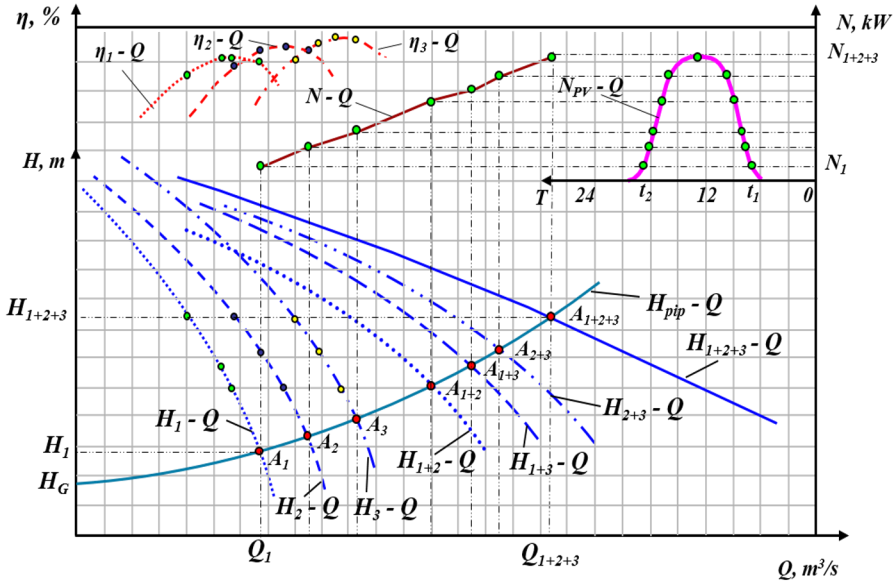
Fig. 2. Graphs of operating modes of three pumps connected in parallel: H_{1,2,3} - Q - 1, 2 and 3 - head characteristics of pumps; H_{1+2,1+3,2+3,1+2+3} - Q - head characteristics of pumps in parallel operation; \eta_{1,2,3} - Q - efficiency of pumps characteristics; N - Q - characteristics of pump power, N_{PV} - Q - power characteristic of PVP.
