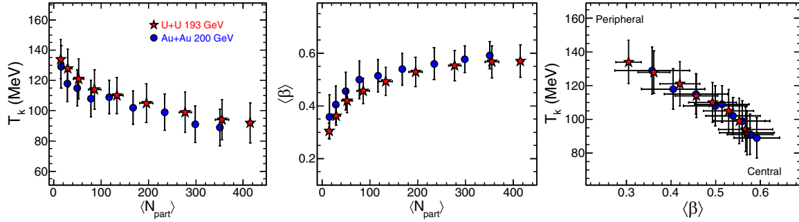
FIG. 10. Left panel: T_k as a function of \langle N_{\text{part}} \rangle . Middle panel: \langle\beta\rangle as a function of \langle N_{\text{part}} \rangle . Right panel: variation of T_k with \langle\beta\rangle . The midrapidity ( |y| < 0.1 ) results from U+U collisions at \sqrt{s_{NN}} = 193 GeV are compared with Au+Au collisions at \sqrt{s_{NN}} = 200 GeV [58]. The uncertainties represent the total systematic and statistical uncertainties added in quadrature, dominated by systematic uncertainties.
