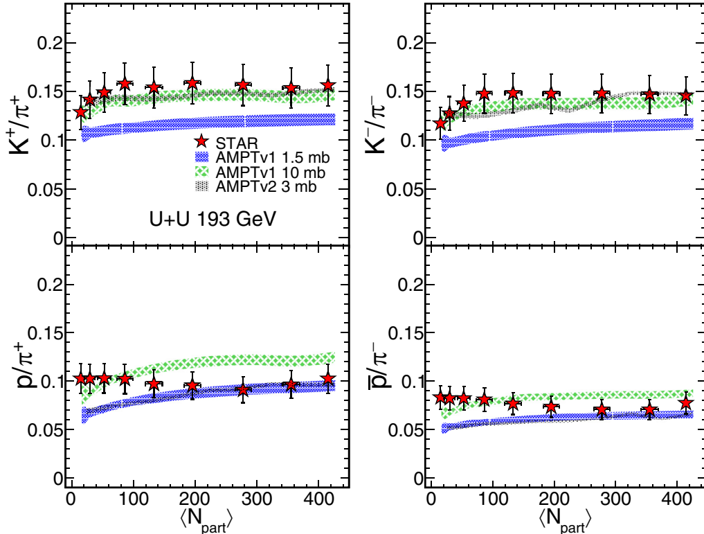
FIG. 14. K^+/\pi^+ , K^-/\pi^- , p/\pi^+ , and \bar{p}/\pi^- particle yield ratios at midrapidity ( |y| < 0.1 ) as a function of \langle N_{\text{part}} \rangle obtained for three calculations of AMPT data (AMPTv1 1.5 mb, AMPTv2 3 mb, and AMPTv1 10 mb) are shown along with the STAR results obtained in U+U collisions at \sqrt{s_{NN}} = 193 GeV. The width of the bands corresponds to the statistical uncertainty associated with the calculation using the AMPT model.
