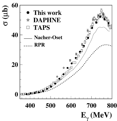
Fig. 4. The total unpolarized cross section for the \gamma p \rightarrow n\pi^+\pi^0 channel obtained in this work is compared to previous DAPHNE [23] and TAPS [25] data. The solid and dashed lines represent the prediction of the Nacher–Oset [9] and the RPR [12,13] models, respectively. Only statistical errors are shown.
