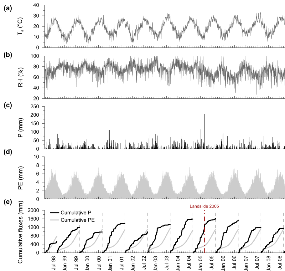
Figure 3. Meteorological variables recorded at the 2005NIL site between January 1998 and August 2008: (a) mean daily air temperature ( T_a ); (b) mean daily air relative humidity (RH); (c) daily precipitations ( P ); (d) daily potential evaporation (PE); (e) precipitation ( P ) and potential evaporation (PE), cumulated during each hydrological year.
