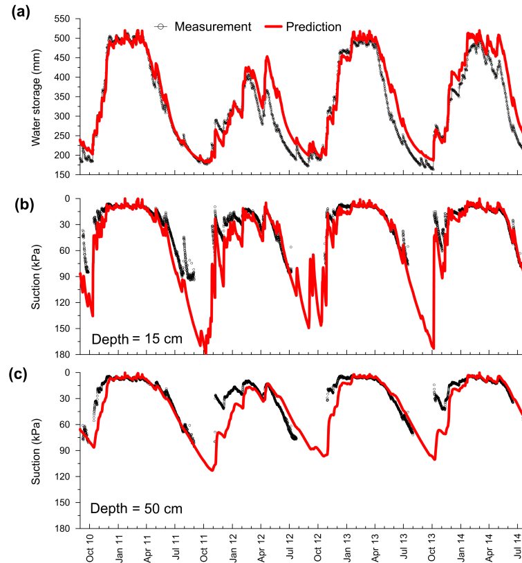
Figure 10. Back analysis of the observed layer hydrological behaviour by the IEM: (a) measured versus IEM-predicted water storage (WS); (b) measured versus IEM-predicted suction at depth of 15 cm; (c) measured versus IEM-predicted suction at depth of 50 cm.
