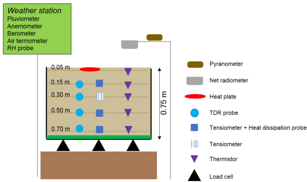
Figure 4. Monitoring devices installed in the physical model (Rianna et al., 2014a, modified).
