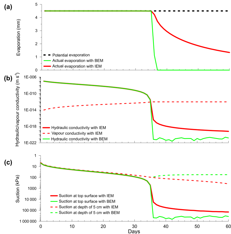
Figure 14. Comparison of variables yielded by IEM and BEM predictions under PE = 4.5 \text{ mm day}^{-1} : (a) comparisons between actual evaporative fluxes (AE); (b) comparisons between hydraulic conductivities at the top surface and evolution of vapour conductivity at the top surface; (c) comparisons between evolutions of suction at the top surface and at depth of 5 cm.
