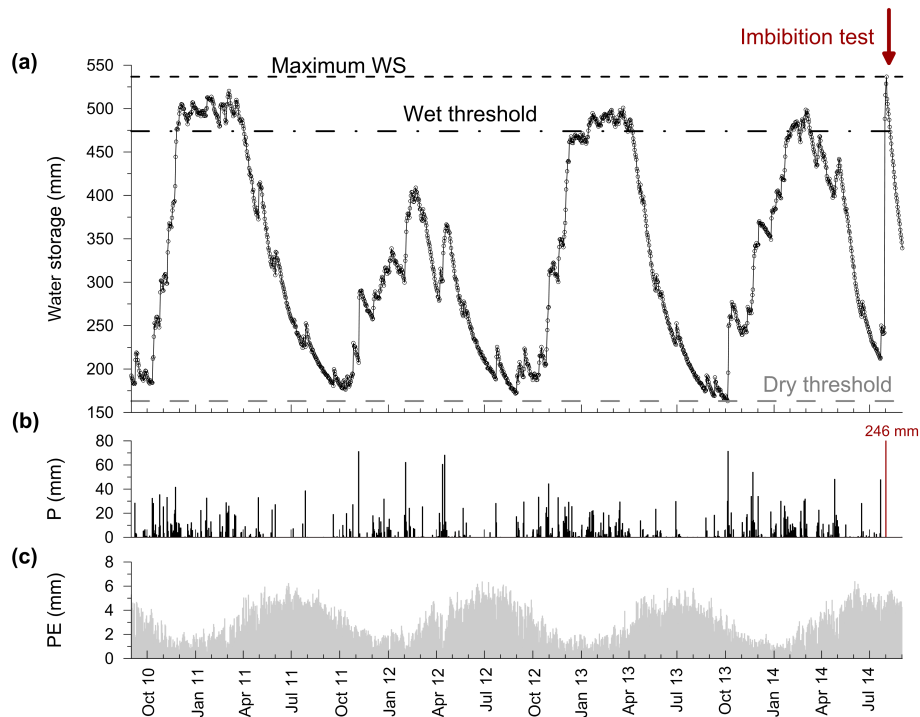
Figure 5. Evolution of variables recorded by the physical model of lysimeter: (a) layer water storage (WS); (b) daily precipitations ( P ); (c) daily potential evaporation (PE). (Records taken over the first 2 hydrological years are from Rianna et al., 2014a.)
