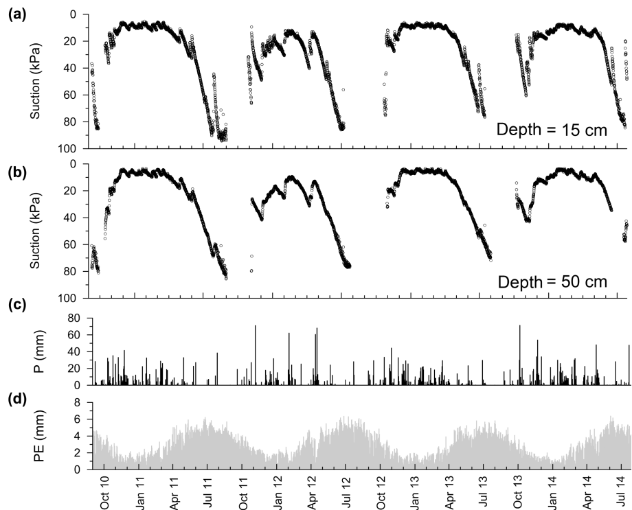
Figure 6. Evolution of variables recorded by the physical model of lysimeter: (a) matric suction at depth of 15 cm; (b) matric suction at depth of 50 cm; (c) daily precipitations ( P ); (d) daily potential evaporation (PE). (Over the first 2 hydrological years records are from Rianna et al., 2014a.)
