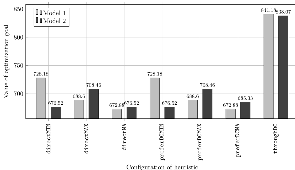
Fig. 6. Optimization goal in function of different heuristic configurations in network polska .
