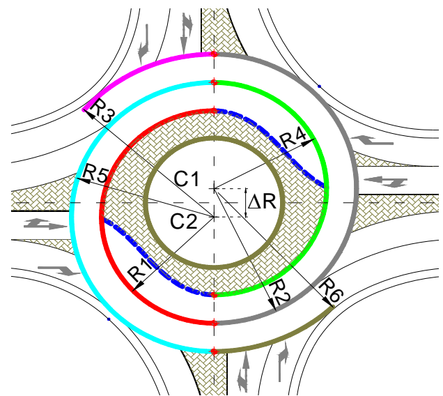
Fig. 3 Geometric design of the turbo roundabout.
