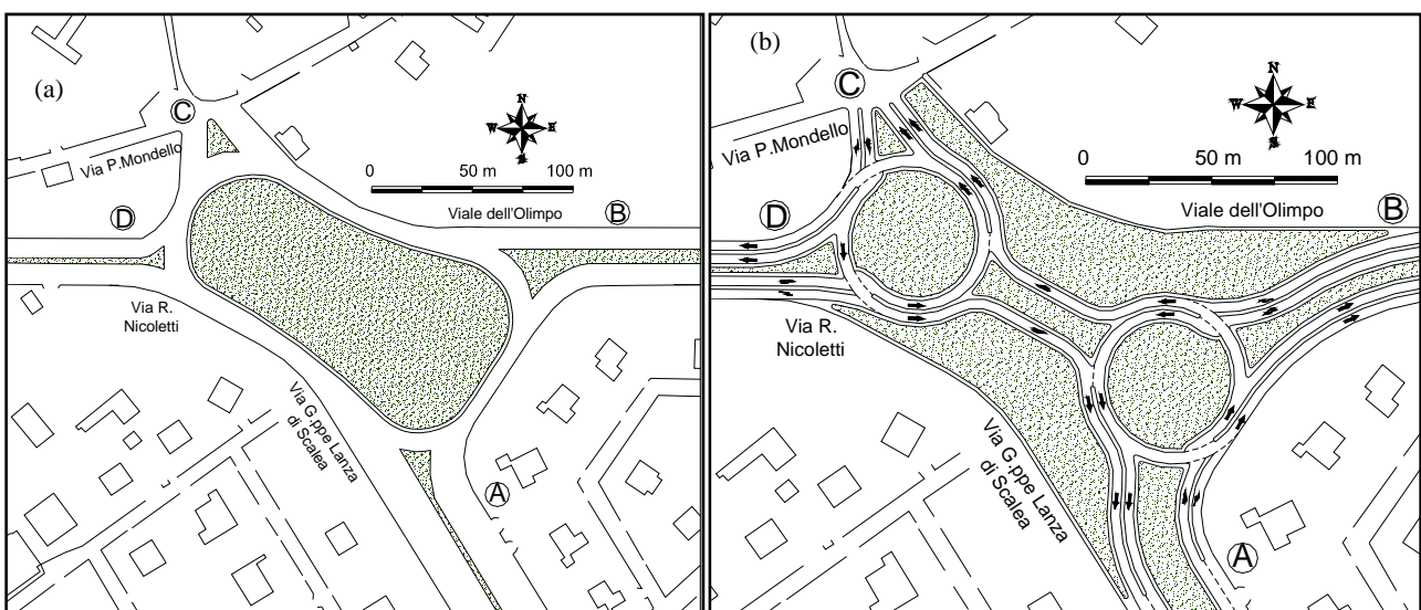
Fig. 9 Characterizes of central island: (a) Present installation; (b) planned scheme of double turbo roundabout.
