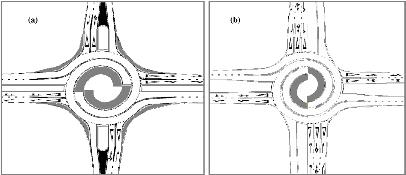
Fig. 1 Two different types of roundabout: (a) A basic turbo roundabout; (b) a spiral roundabout.
