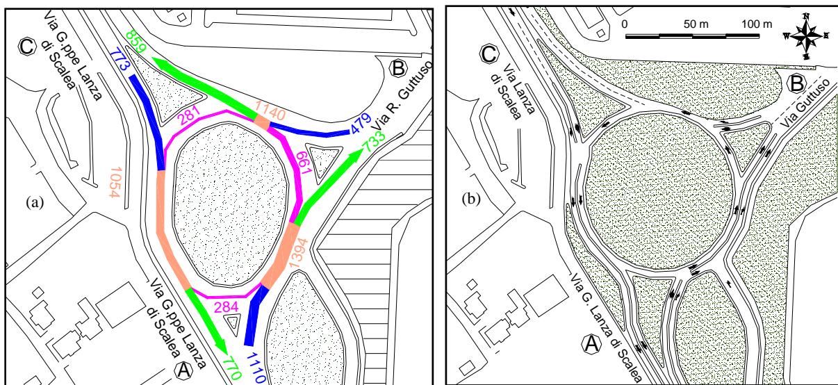
Fig. 8 El Alamein Fallen Square: (a) the existing situation with traffic flows (time interval 18:30-19:30); (b) the planned solution (turbo roundabout with two circulating lane).
