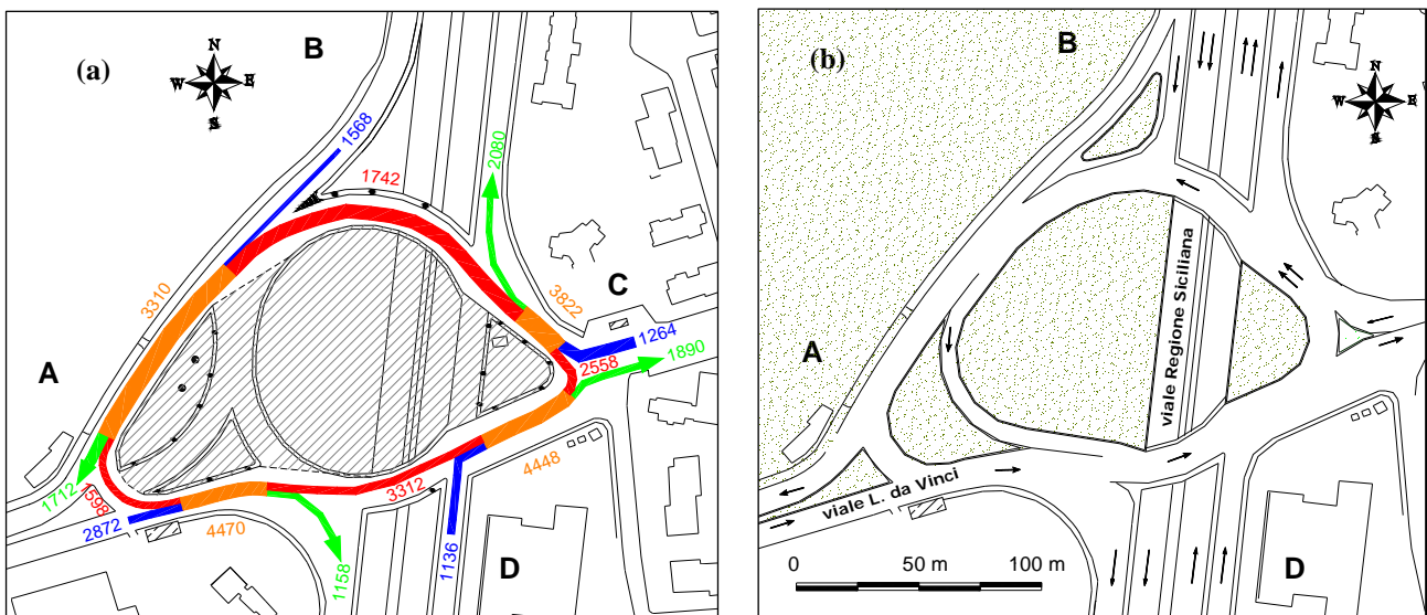
Fig. 7 Einstein Square: (a) the existing situation with traffic flows (time interval 8:30–9:30); (b) the planned solution.
