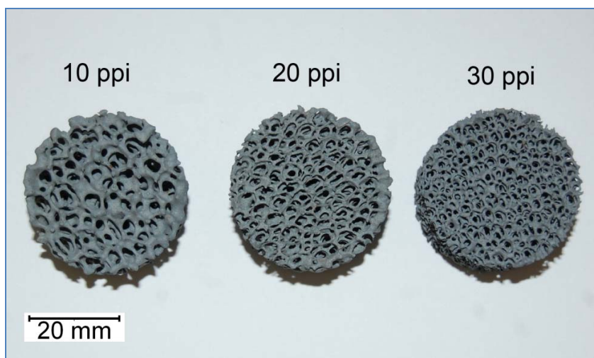
Figure 1: Beta-SiC filters having different porosity.
