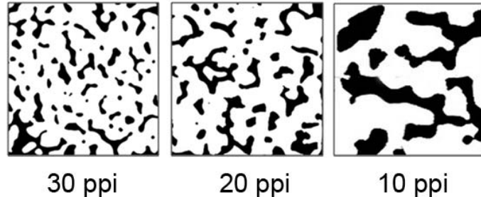
Figure 4: Examples of image processing for density and surface-volume ratio calculations.
