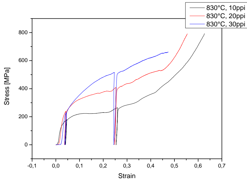
Figure 7: Strain-stress records from DP500 foam compression testing.
