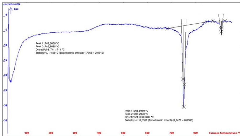
Figure 2: DSC report from DP500 alloy.
