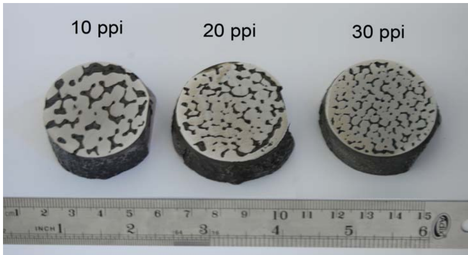
Figure 3: Dual phase steel foams having different porosity.
