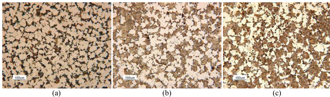
Figure 6: DP500 microstructures. Quenching temperature: (a) = 770 °C, (b) = 800 °C, and (c) = 830 °C.
