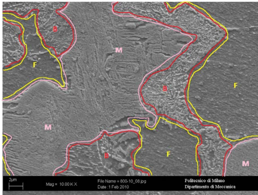
Figure 5: DP500 microstructure. Quenching temperature = 800 °C.
