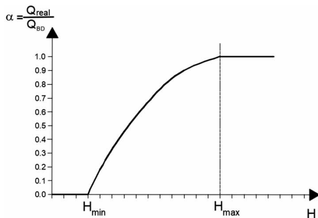
Figure 1 | Value of Q_{real} from each node in the PDA condition.
