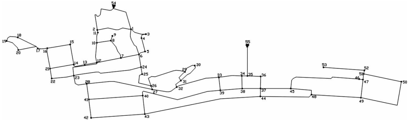
Figure 3 | Network of Praia a Mare (CS, Italy).
