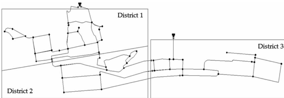
Figure 4 | Initial condition: eight shut-off valves and three districts (Praia a Mare).
