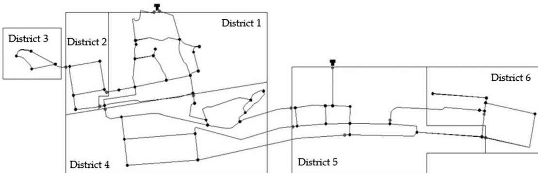
Figure 5 | Scenario n°6: 14 shut-off valves and 6 districts (Praia a Mare).
