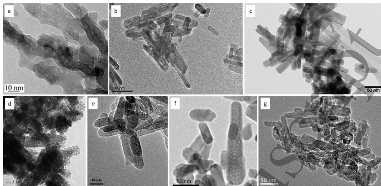
Fig 10: Mesoporous HA with physiologic-like shape obtained through different templating agents: a-c) CTAB [17,50,53], d-e) Pluronic F127 [27,55], f) Triton X-100 [24] and g) Tea polyphenols [58]. All images are reproduced with permission.
