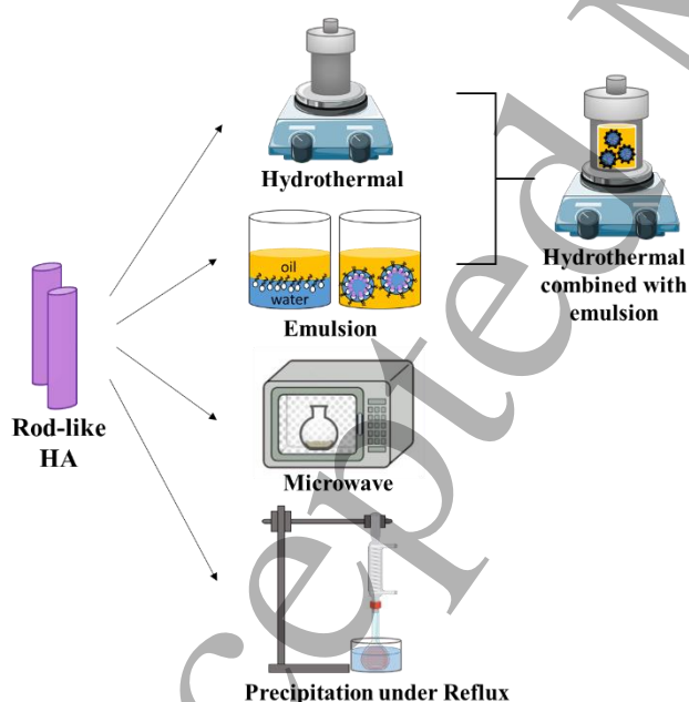
Fig 6: Schematic representation of the synthesis methods suitable for the production of rod-like HA
