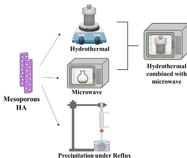
Fig 9: Schematic representation of the synthesis methods suitable for the production of mesoporous HA.
