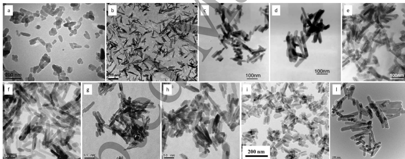
Fig 7: Rod-like HA particles obtained by different authors: a) Iyyappan et al. [25], b) Wang et al. [32], c-d) Wang et al. [33], through hydrothermal treatment at 120° C for 24 h and at 150° C for 20 h, e) Yan et al. [34], f-h) Wang et al. [37], with PEG, trisodium citrate and Tween 20, i) Xin et al. [35] and l) Lin et al. [39]. All images are reproduced with permission.
