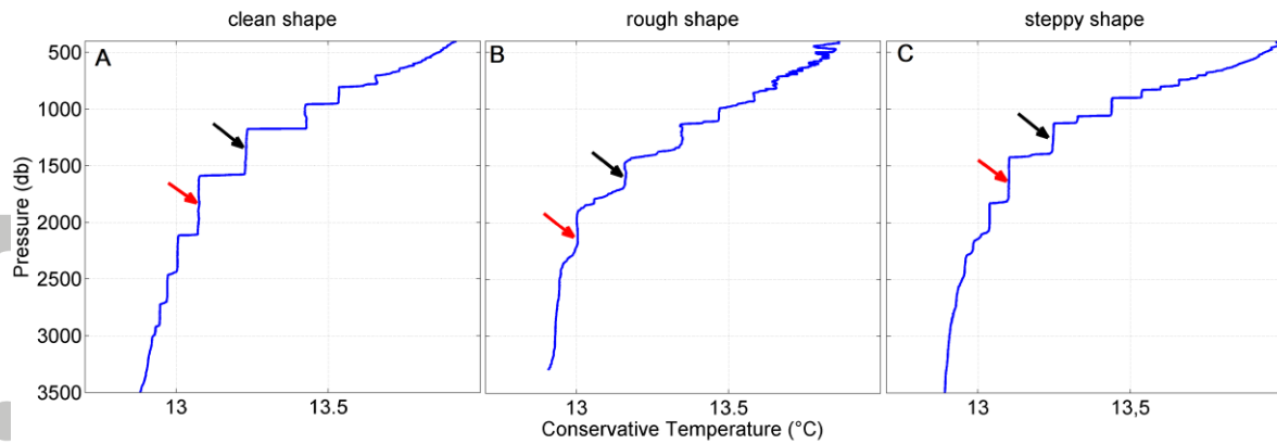
Figure 2. (A): A "clean" profile characterized by a high number of recognizable steps, with high thicknesses and very well-mixed layers, very thin interfaces and also smaller, secondary steps at the top and at the bottom of the staircase zone. (B): A "rough " profile characterized by few thick steps alternated by sloped and rough interfaces. (C): A "steppy" profile characterized by thin interfaces embedding sub-steps. Red arrows indicate the "main" step, black arrows the "middle" step.
