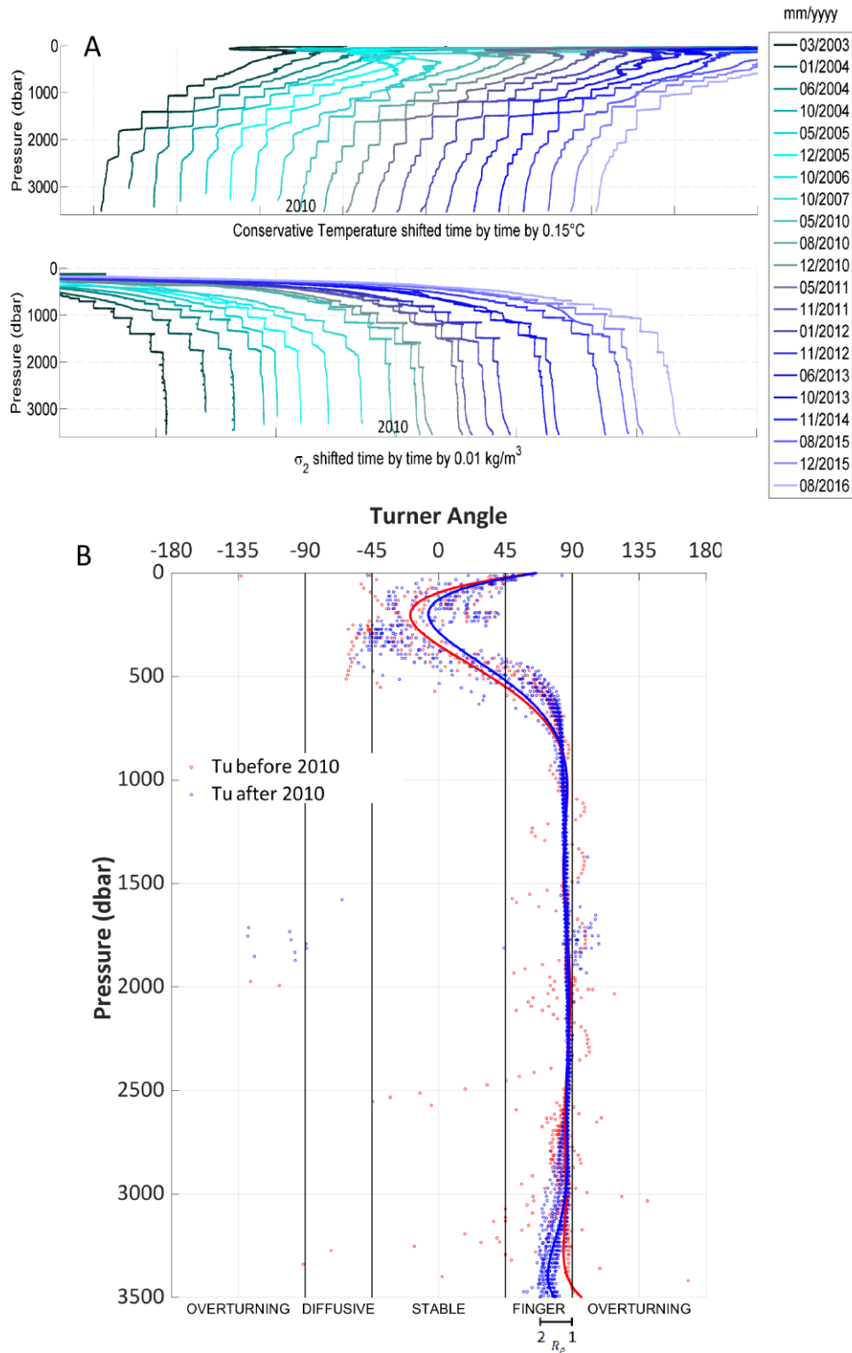
Figure 3. (A): Conservative Temperature and Sigma-2 profiles shifted in time for a better visualization. The slight density inversions in the first three profiles are due to hydrological cable issue. After 2010 it becomes visible the presence of a denser water at the bottom of the Sigma-2 profiles. (B): Scatter plot of the Tu along the water column before (red dots) and after (blue dots) 2010. Best fit curves of Tu vs pressure, shown in the same colors, are calculated with a 8-th order polynomial using the Matlab Curve fitting toolbox.
