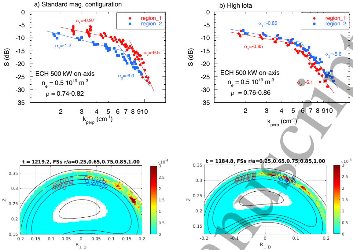
FIG. 6: Upper row: Experimental k_{\perp} spectra measured in two plasma regions poloidally separated (see Fig. 1 caption for the explanation of regions) in the standard (left) and high iota (right) magnetic configurations. Lower row: EUTERPE simulation of the localization of the instabilities for the standard (left) and high iota (right) magnetic configurations. Red and blue circles indicate the left and right DR probing regions, respectively.
