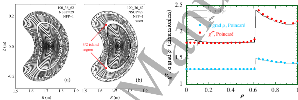
FIG. 8: Left: A TJ-II magnetic configuration perturbed by a small error field. Right: Comparison between some metric coefficients computed using the analytical annular model with island width 1.7 cm (continuous lines) and numerically obtained from the Poincaré plot with islands in the left part of the figure (dots). (Reproduced from [49] with permission of the Journal).
