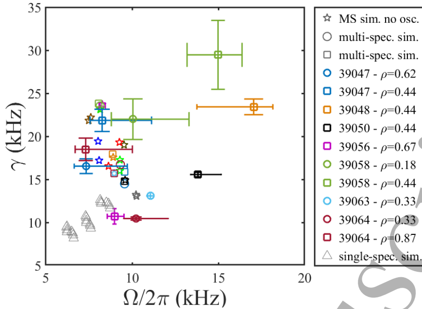
FIG. 5: Damping rate ( \gamma ) vs oscillation frequency ( \Omega ) for the experimental oscillations detected in [28]. Data are shown for the specified TJ-II discharges and for numerical simulations, both with a single (grey triangles) and with multiple kinetic species, namely hydrogen ions+electrons+C 4+ impurity ions (circles, squares and pentagrams) [29]. The same color is used for experimental points (showing error bars) and for multi-species simulated discharges (without error bars). Note that some plotted discharges showed no oscillations (pentagrams). For some discharges with insufficient profile data, profiles from a similar discharge were used in the simulation. In the first three rows of the legend, symbols are shown with a single grey color to avoid an excessive legend length. The multi-species simulation data in this figure are corrected relative to a previous version in Figure 13 from [29].
