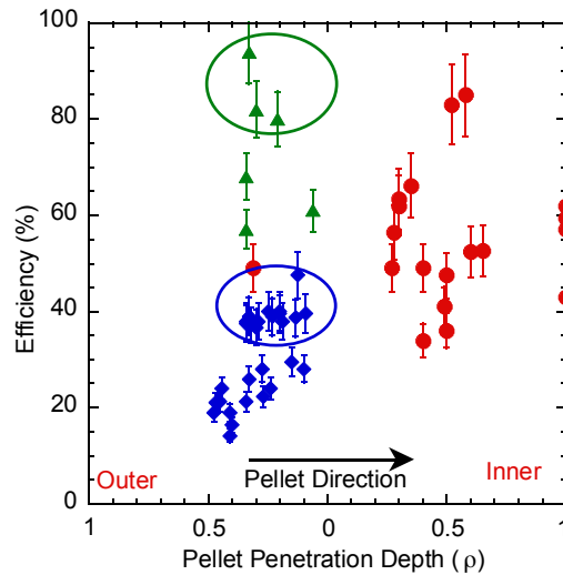
FIG. 10: Fuelling/deposition efficiency as a function of pellet penetration depth into TJ-II standard configuration plasmas. The data are for cryogenic hydrogen (filled blue diamonds) and polystyrene (green triangles) pellets injected into ECRH plasmas and cryogenic hydrogen pellets (red dots) injected into NBI plasmas. Cases for which a population of fast electrons is present in the core during pellet injection are contained within the ovals. Examples of pellets that are not fully ablated within the plasma are plotted on the right axis.
