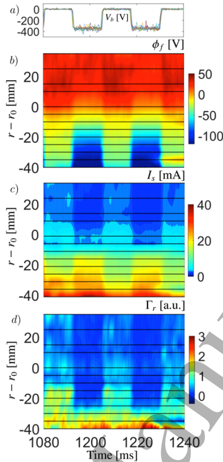
FIG. 7: a) Biasing voltage waveform; b), c) and d) Radial profiles of floating potential, ion saturation current and turbulent flux, respectively, during dynamical biasing in the plasma boundary region. r - r_0 < 0 corresponds to the plasma edge; r - r_0 > 0 corresponds to the SOL.
