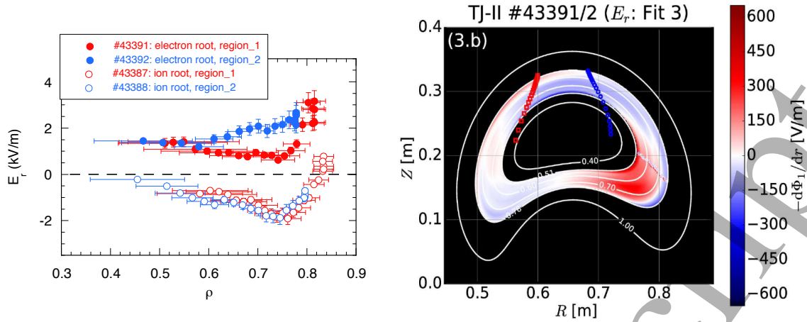
FIG. 2: Left, E_r profiles measured by the Doppler reflectometer at turbulence scales k_\perp \sim 6 - 8 \text{ cm}^{-1} , in the two plasma regions (1 in red and 2 in blue) in both electron and ion root regimes. Right, calculated contribution to the radial electric field component that arises from the radial dependency of \varphi_1 . Plasma regions 1 and 2 are indicated by consistently coloured thick lines in the upper (external) part of the plasma cross section.
