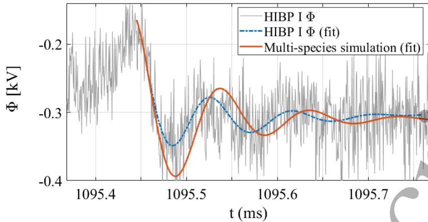
FIG. 4: Comparison of a potential relaxation experimentally measured by the HIBP diagnostic in plasma discharge 39063, the corresponding fit (in blue) and the fit of multi-ion simulated relaxation (in orange) to a damped oscillatory model (including the correction to the frequency introduced by the formula 21 from [29]).
