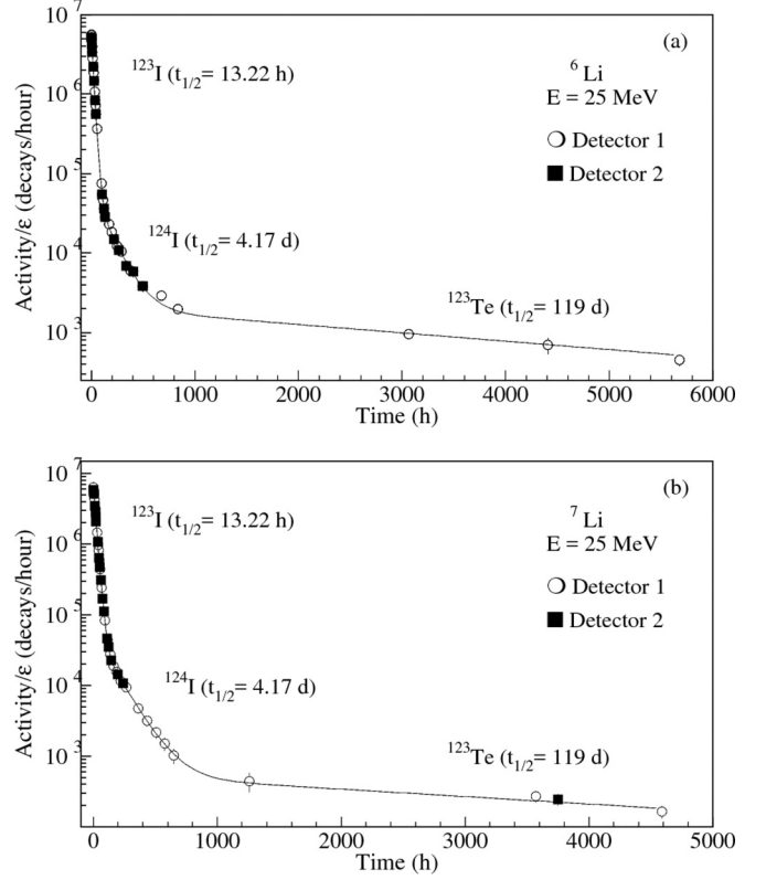
FIG. 3. Typical activity curves (a) for the {}^6\text{Li} + {}^{120}\text{Sn} reaction and (b) for the {}^7\text{Li} + {}^{119}\text{Sn} reaction. The continuous line is the best fit of the activity curve.
