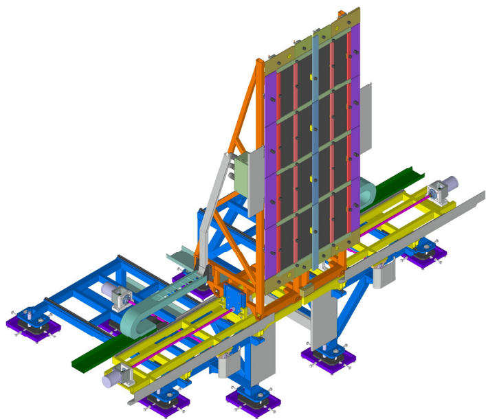
Figure 5 CAD model of STRIKE; front surface hit by the beam is shown
