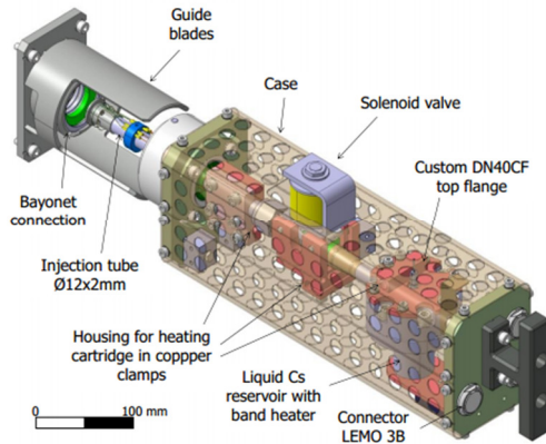
Figure 2 Caesium oven 3D view.
