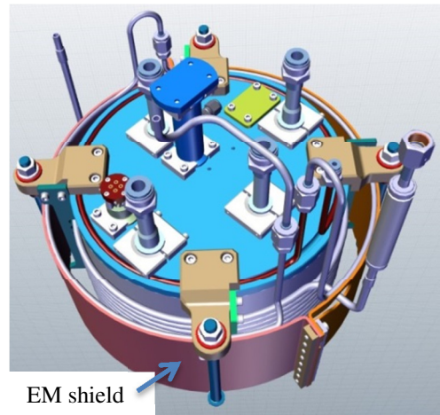
Figure 3 Rf driver with EM shield.
