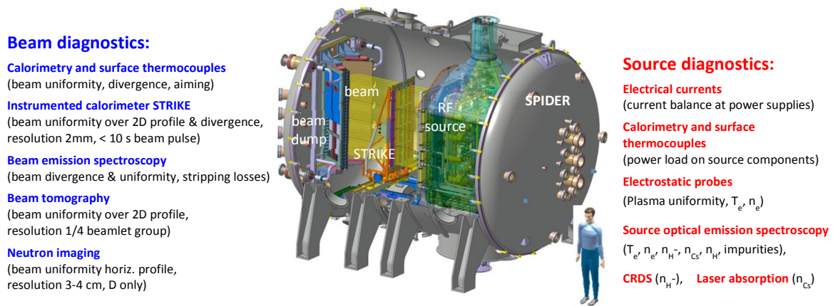
Figure 4 SPIDER in-vessel view and list of source and beam diagnostics with measured parameters
