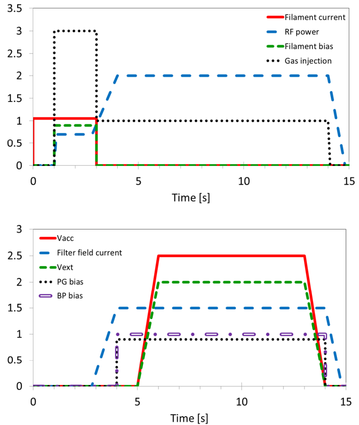
Figure 8 Sketch of the time traces of the main control parameters of SPIDER operation; arbitrary units are used
