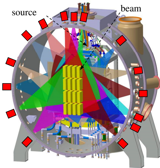
Figure 6 Vertical cross-section of the SPIDER vessel with view of the 4x4 beamlet groups and 15 linear cameras of the tomographic diagnostic with corresponding fans of lines of sight
