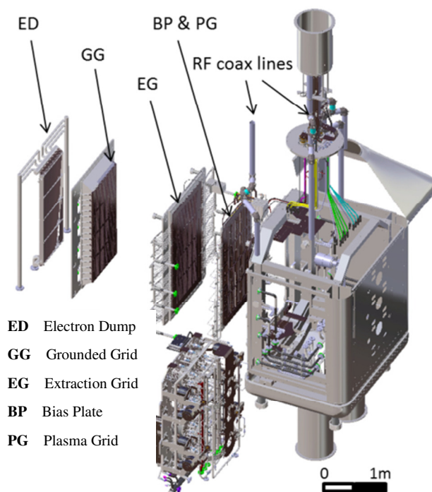
Figure 1 Beam Source 3D exploded view.
