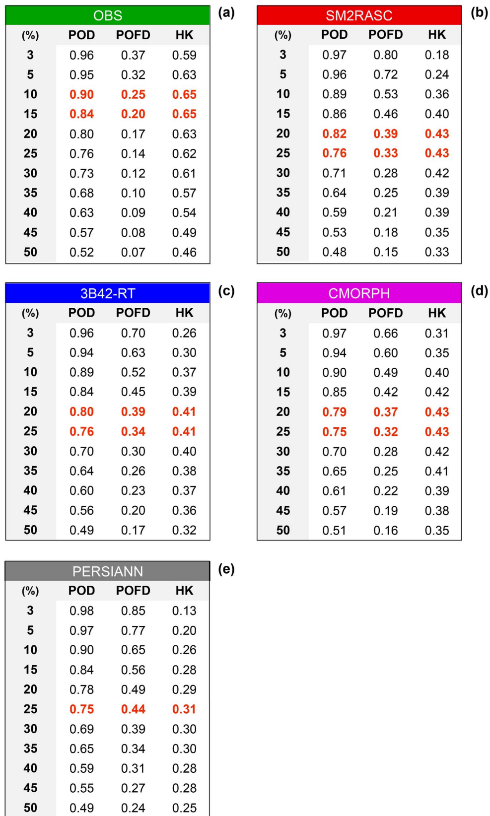
Fig. 6. Values of the POD, POFD and HK skill scores obtained varying the threshold non-exceedance probability for the five data sets. Values in red are those that maximize HK. (For interpretation of the references to color in this figure legend, the reader is referred to the web version of this article.)
