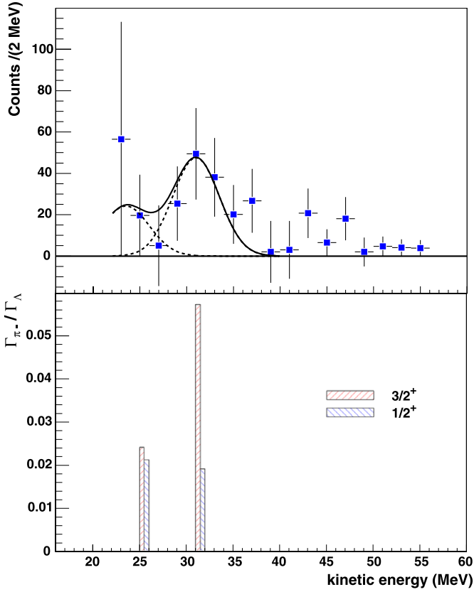
Fig. 6. Upper part: kinetic energy spectrum of MWD \pi^- for {}^{15}_{\Lambda}\text{N} after acceptance correction. The solid curve is a two-gaussian fit to the peaks in the spectrum, to compare with theoretical predictions in the lower part; dashed curves are the single components. Lower part: calculated major decay rates to final {}^{15}\text{O} states from [18], in red bars for {}^{15}_{\Lambda}\text{N} ground-state spin-parity 3/2^+ , and in blue bars for {}^{15}_{\Lambda}\text{N} ground-state spin-parity 1/2^+ . Note that in this case the arbitrary bar width was reduced to 0.5 MeV to avoid overlap and to facilitate the comparison between the two spin hypotheses: indeed, the energies of the produced final states are practically the same. (For interpretation of the references to color in this figure legend, the reader is referred to the web version of this article.)
