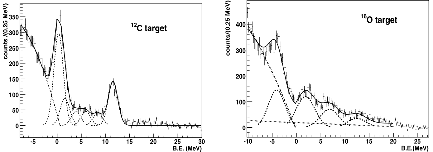
Fig. 1. Inclusive binding energy spectra for good quality \pi^- tracks coming from ^{12}\text{C} (left) and ^{16}\text{O} (right) targets. The continuous line is the best fit curve to the spectra; the dashed curves represent the contributions from the known hypernuclear states and the dot-dashed curve the \Lambda_{qf} background. For ^{16}\text{O} the dotted curve parametrizes the K^- decay in flight.
