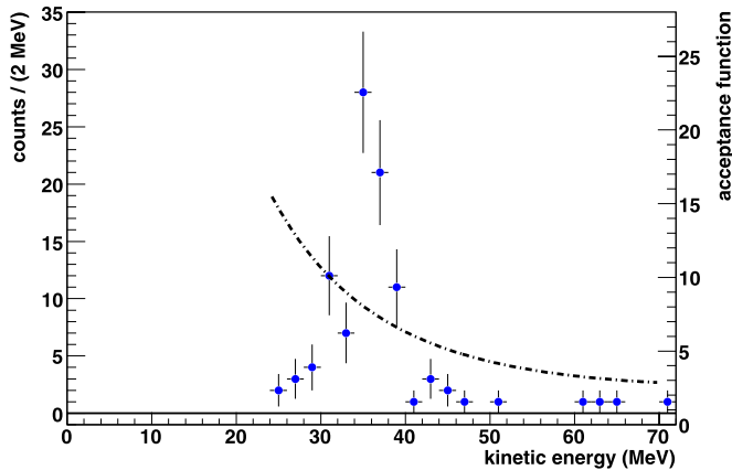
Fig. 2. Kinetic energy spectrum of MWD \pi^- for {}^7\text{Li} before acceptance correction. The dot-dashed curve is the acceptance function, \bar{R} , to be applied to the data.
