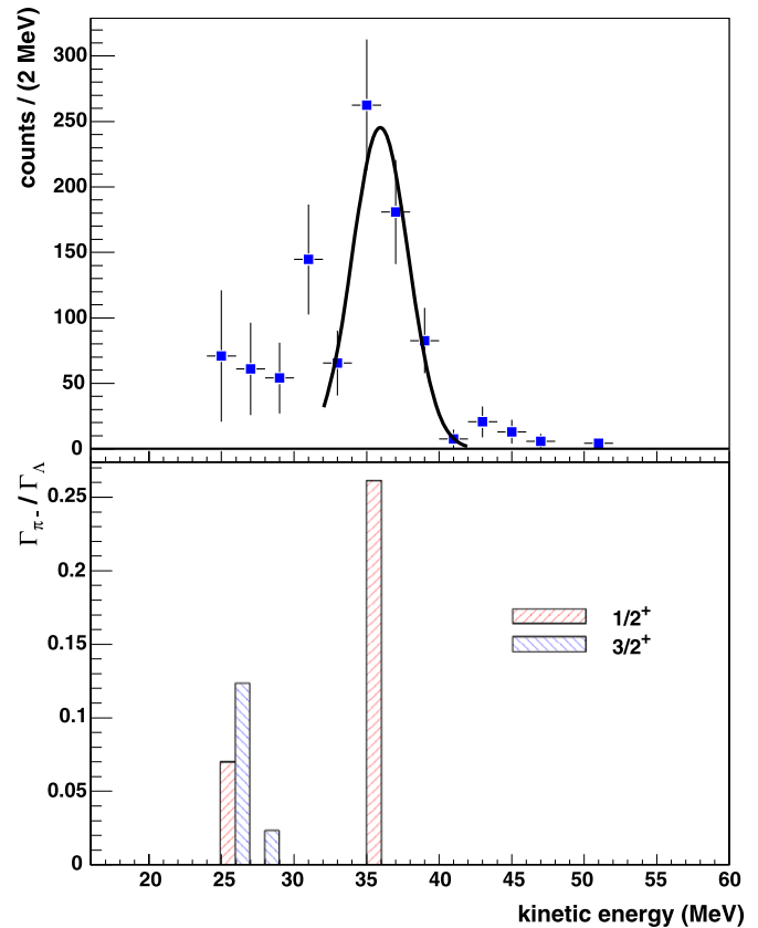
Fig. 3. Upper part: kinetic energy spectrum of MWD \pi^- for {}^7\text{Li} after acceptance correction. The solid curve is a gaussian fit to the peak in the spectrum, to compare with theoretical predictions in the lower part. Lower part: calculated major decay rates to final {}^7\text{Be} states from [18], in red bars for {}^7\text{Li} ground-state spin-parity 1/2^+ , and in blue bars for {}^7\text{Li} ground-state spin-parity 3/2^+ (see text). (For interpretation of the references to color in this figure legend, the reader is referred to the web version of this article.)
