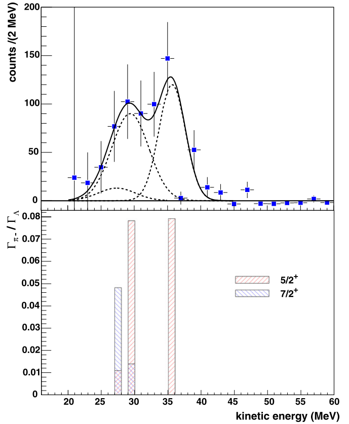
Fig. 5. Upper part: kinetic energy spectrum of MWD \pi^- for {}^{11}\text{B} after acceptance correction. The solid curve is a two-gaussian fit to the peaks in the spectrum, to compare with theoretical predictions in the lower part; dashed curves are the single components. Lower part: calculated major decay rates to final {}^{11}\text{C} states from [18], in red bars for {}^{11}_A\text{B} ground-state spin-parity 5/2^+ , and in blue bars for {}^{11}_A\text{B} ground-state spin-parity 7/2^+ . (For interpretation of the references to color in this figure legend, the reader is referred to the web version of this article.)
