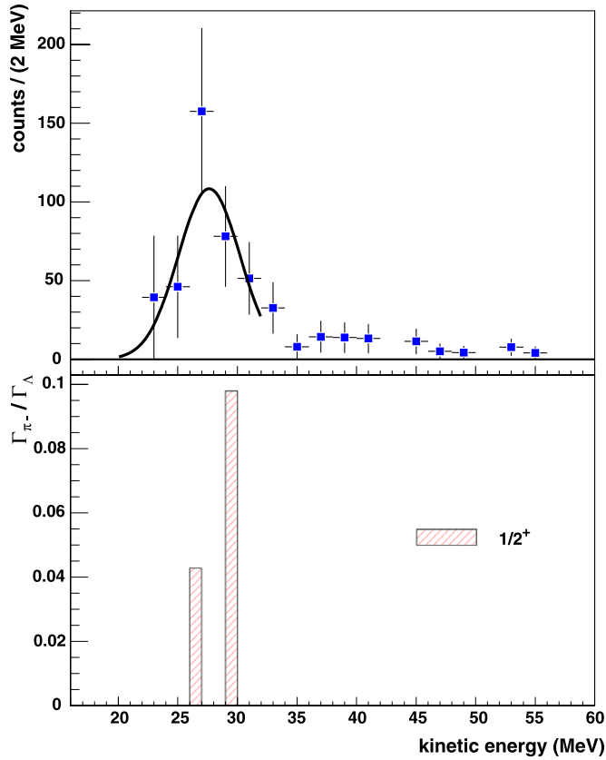
Fig. 4. Upper part: kinetic energy spectrum of MWD \pi^- for {}^9\text{Be} after acceptance correction. The solid curve is a gaussian fit to the peak in the spectrum, to compare with theoretical predictions in the lower part. Lower part: calculated major decay rates to final {}^9\text{B} states from [18], in red bars for {}^9\text{B} ground-state spin-parity 1/2^+ . (For interpretation of the references to color in this figure legend, the reader is referred to the web version of this article.)
