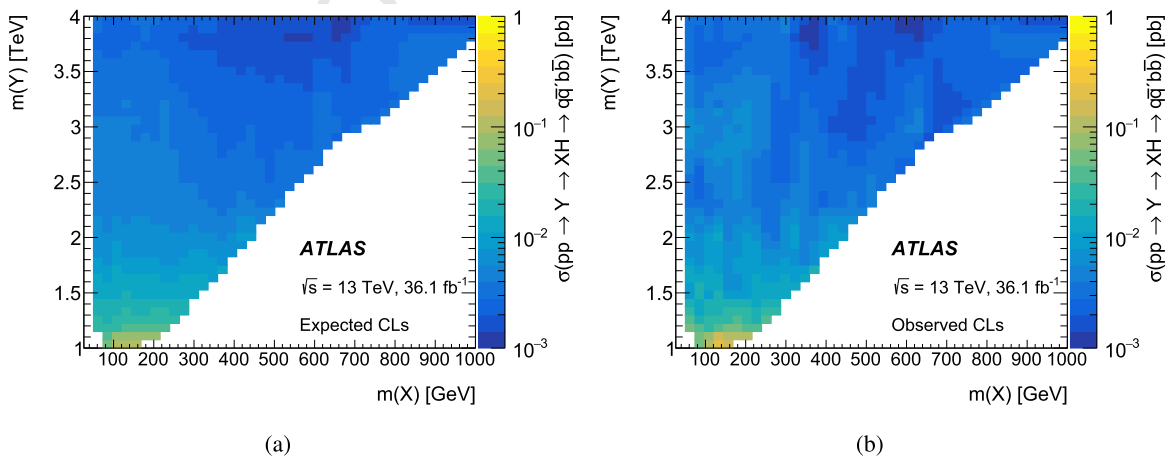
Fig. 6. The (a) expected and (b) observed 95% CL limits on the production cross-section \sigma(pp \rightarrow Y \rightarrow XH \rightarrow qq'bb) (z-axis) in the two-dimensional space of m(Y) versus m(X) . (For interpretation of the references to colour in this figure, the reader is referred to the web version of this article.)
