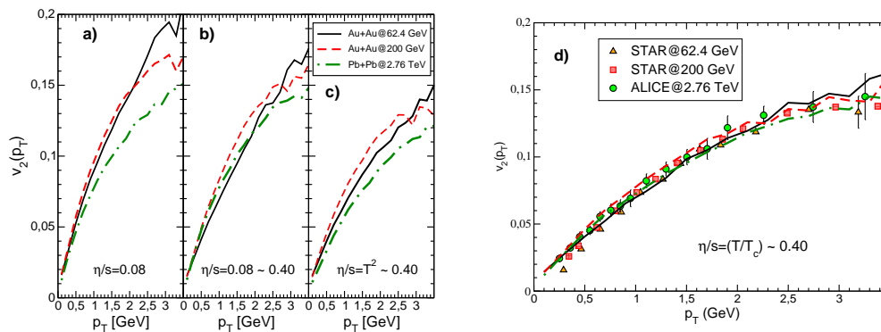
Figure 2. v_2(p_T) at mid rapidity for 10% – 20% collision centrality. The solid line, the dashed line and the dot dashed line refer to: Au + Au at \sqrt{s} = 62.4 GeV and \sqrt{s} = 200 GeV and Pb + Pb at \sqrt{s} = 2.76 TeV, respectively for different behavior of \eta/s(T) as indicated in the labels.
