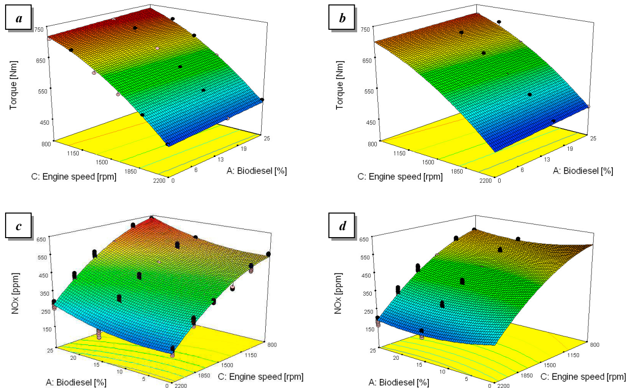
Figure 2 – Surface plot of the engine torque (a and b) and the NO x concentration in the exhaust gases (c and d) as a function of the biodiesel percentage and of the engine speed, with the 0 % (a and c) and the 3 % (b and d) of bioethanol in the blend.
