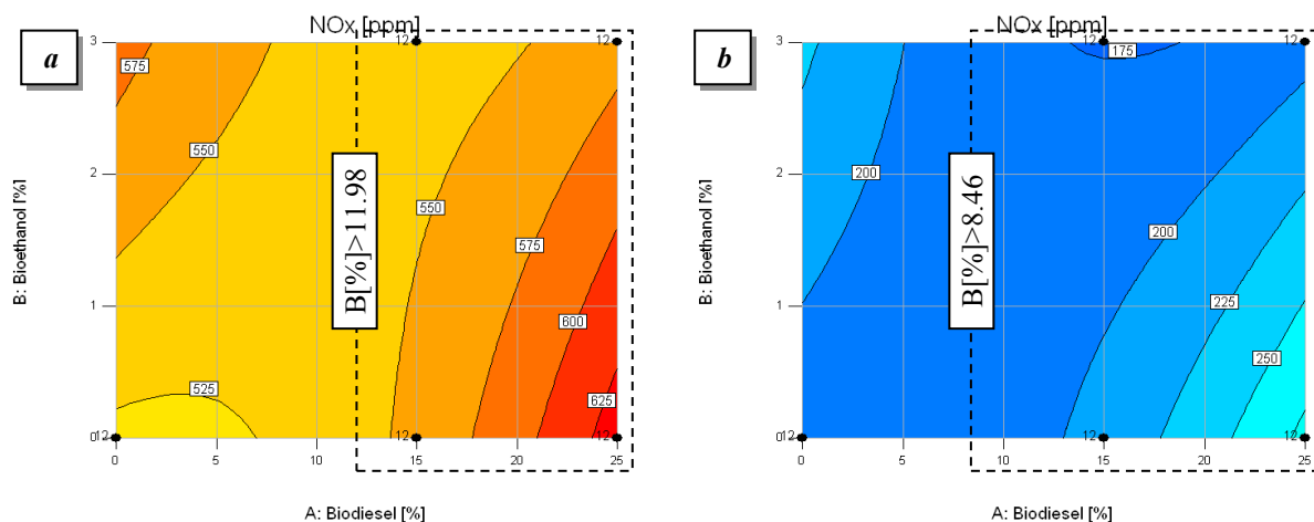
Figure 3 – Contour plots of the NOx concentration as a function of the bioethanol and biodiesel percentages (full ranges of concentration), at 1121 rpm (a) and 2991 rpm (b); the values of NOx are reported as labels directly on the contours.
