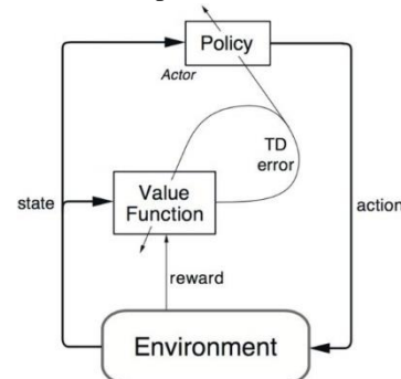
FIGURE 1. Reinforcement learning architecture
