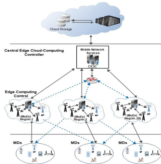
FIGURE 2. High-level overview of computation offloading in MEC model
