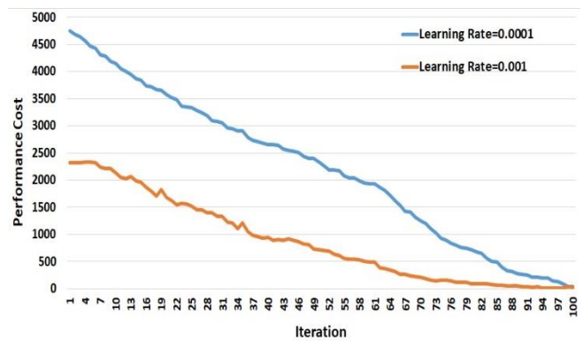
FIGURE 5. DO-SARSA performance under different learning rates
