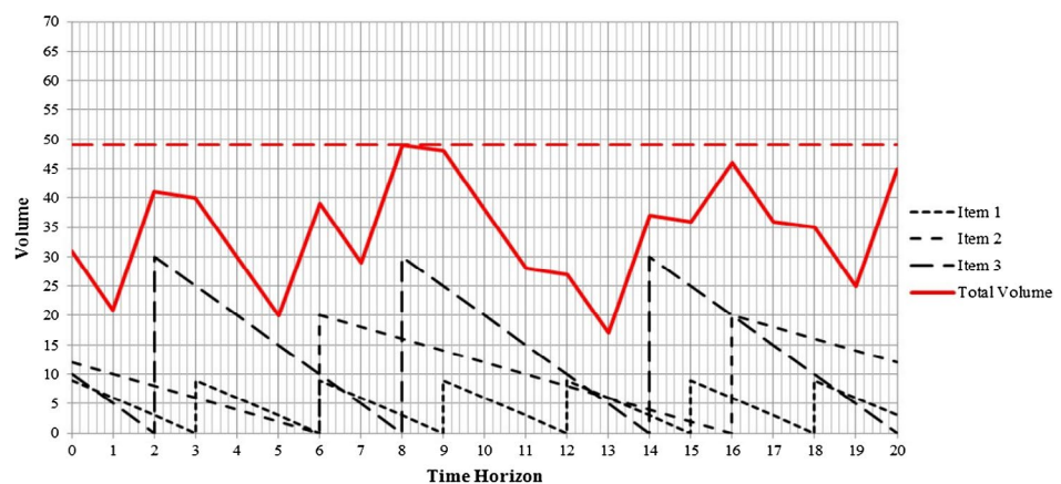
Figure 2. Space requirement with offsetting.
