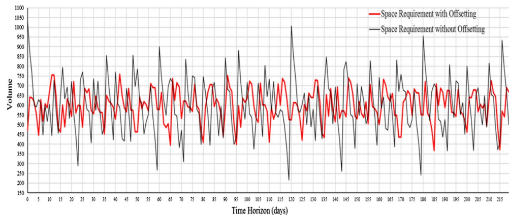
Figure 5. Murthy et al. Case. Comparison between the space requirement with and without offsetting.
