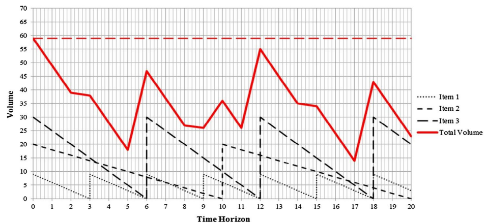
Figure 1. Space requirement without offsetting.
