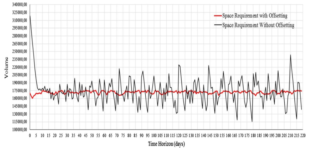
Figure 6. 1,000 item case. Comparison between the space requirement with and without offsetting.
