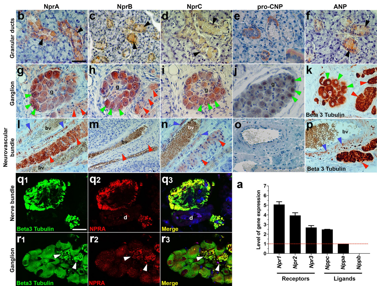
Fig. 1 Expression of the natriuretic peptide system in mouse adult submandibular salivary glands. a RT-qPCR for Npr1 , Npr2 , Npr3 , Nppa , Nppb and Nppc encoding respectively the three natriuretic receptors NprA, NprB and NprC and the three natriuretic ligands ANP, BNP and CNP in male mSMGs. The lowest gene expression ( Nppa ) is represented as one. Expression of other genes was compared to Nppa expression. b–p Immunohistochemistry for NprA ( b , g , l ), NprB ( c , h , m ), NprC ( d , i , n ), CNP ( e , j , o ), ANP ( f ) and beta III tubulin ( k , p ). b–d , f The three receptors and ANP are present in granular ducts. Note a minority of granular duct cells are devoid of immunoreactivity. e Immunostaining for CNP is observed in striated ducts and not granular ducts. An enlargement of a stained striated ducts is presented in the lower right corner showing staining concentrated in the basal striations. g–i The three receptors are present in
