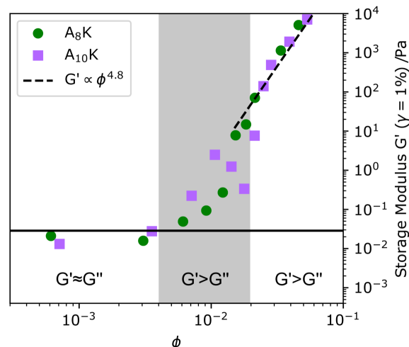
Fig. 4 The scaling behavior of G' as a function of the volume fraction \phi . The G' values were extracted from frequency sweeps at \omega = 1 \text{rads}^{-1} and \gamma = 1 %. The dashed line shows a fit to the high concentration data resulting in G' \propto \phi^{4.8} . The three regions of different viscoelastic properties are highlighted.
