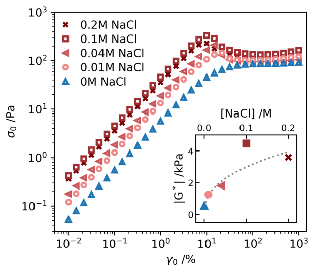
Fig. 7 The stress amplitude, \sigma_0 , as a function of the strain amplitude, \gamma_0 , and salt concentration for a \phi = 0.025 A 10 K sample and at an oscillation frequency \omega = 1 \text{rads}^{-1} . Upon the addition of salt a yield stress is built up due to the transition from repulsive to attractive interactions. The insert shows |G^*| versus the salt concentration as determined from the \sigma_0/\gamma_0 in the linear viscoelastic regime. |G^*| increases roughly an order of magnitude with the salt concentration and eventually levels off. The line in the insert is added as a guide to the eye.
