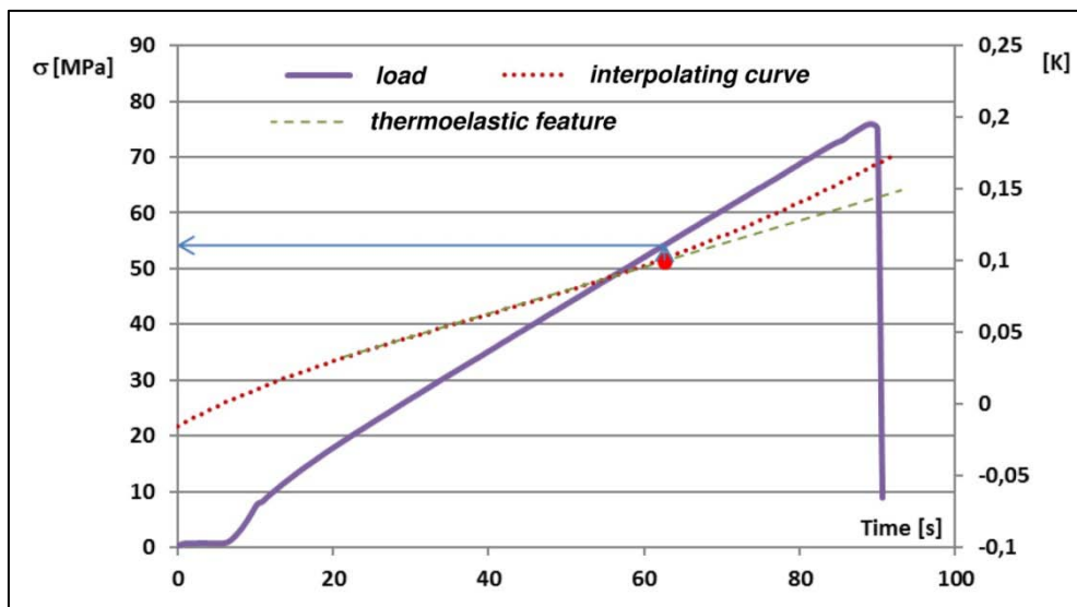
Fig. 4 interpolating curve ( \Delta T-t ) for specimen 2 and diagram ( \sigma-t ) for the spot n.2
