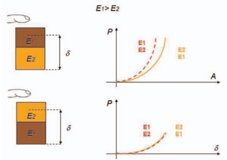
Fig. 1. An object comprised of two layers of different materials is probed for softness from the two sides. The resultant force-displacement ( P/\delta ) curve is equal, while the force-area ( P/A ) curve is steeper when the stiffer layer is above.
