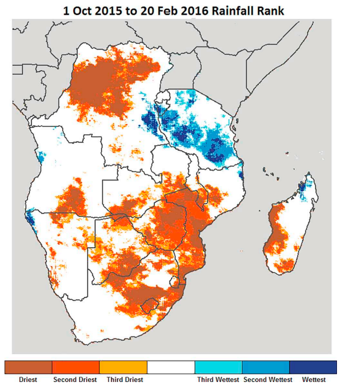
Fig. 5. CHIRPS rainfall ranking for the period 1 October 2015 to 20 February 2016.
