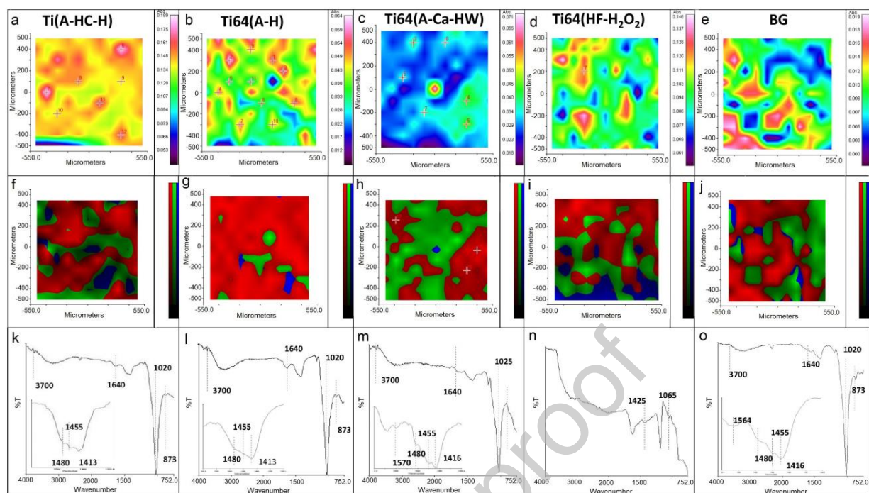
Figure 6: FTIR chemical imaging: chemical map (a-e); PCA analysis (f-j); spectra (k-o) of Ti(A-HC-H), Ti64(A-H), Ti64(A-Ca-H-W), Ti64(HF-H 2 O 2 ), BG samples soaked for 1 day, respectively. Three different scores of PCA analysis, corresponding to different percentages of the spectra data groupings of similar variability, are showed in red, green and blue colors.
