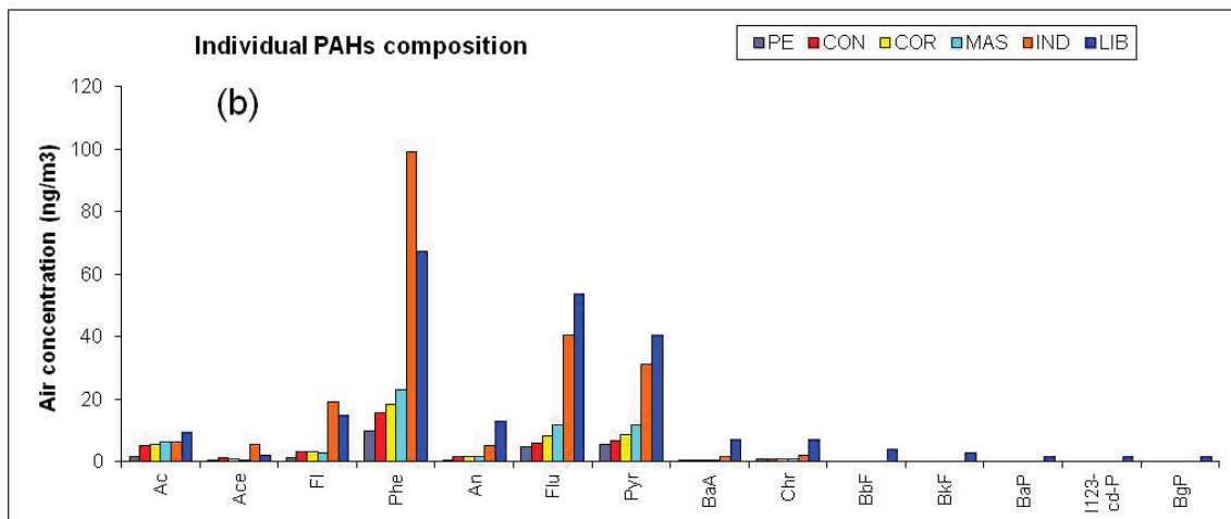
Figure 4. Fraction of individual PAHs (a) and air concentrations (ng m -3 ) (b) and at different sites in Concepción.
