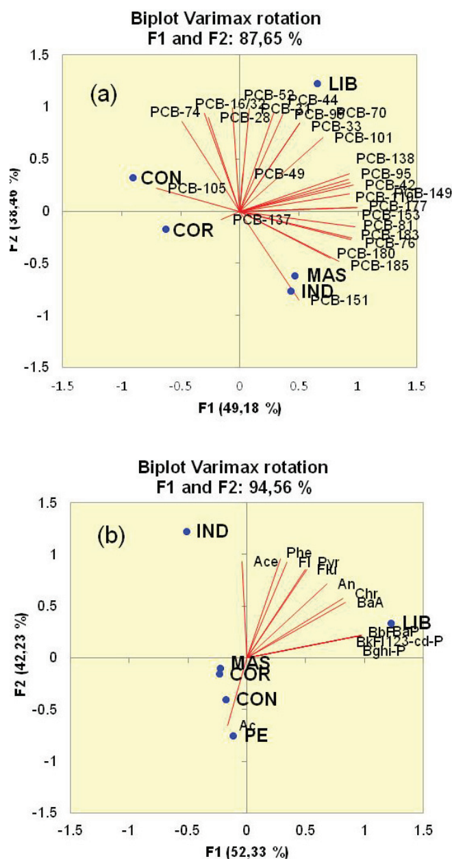
Figure 2. Score plot for principal component analysis (PCA) applied to air measurements across sampling sites in Concepción. (a) PCA analysis of PCBs congeners ( n=26 compounds) and (b) PCA analysis of PAHs ( n=15 ) in Concepción.
