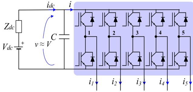
Fig. 1 Circuit scheme of the considered five-phase VSI
